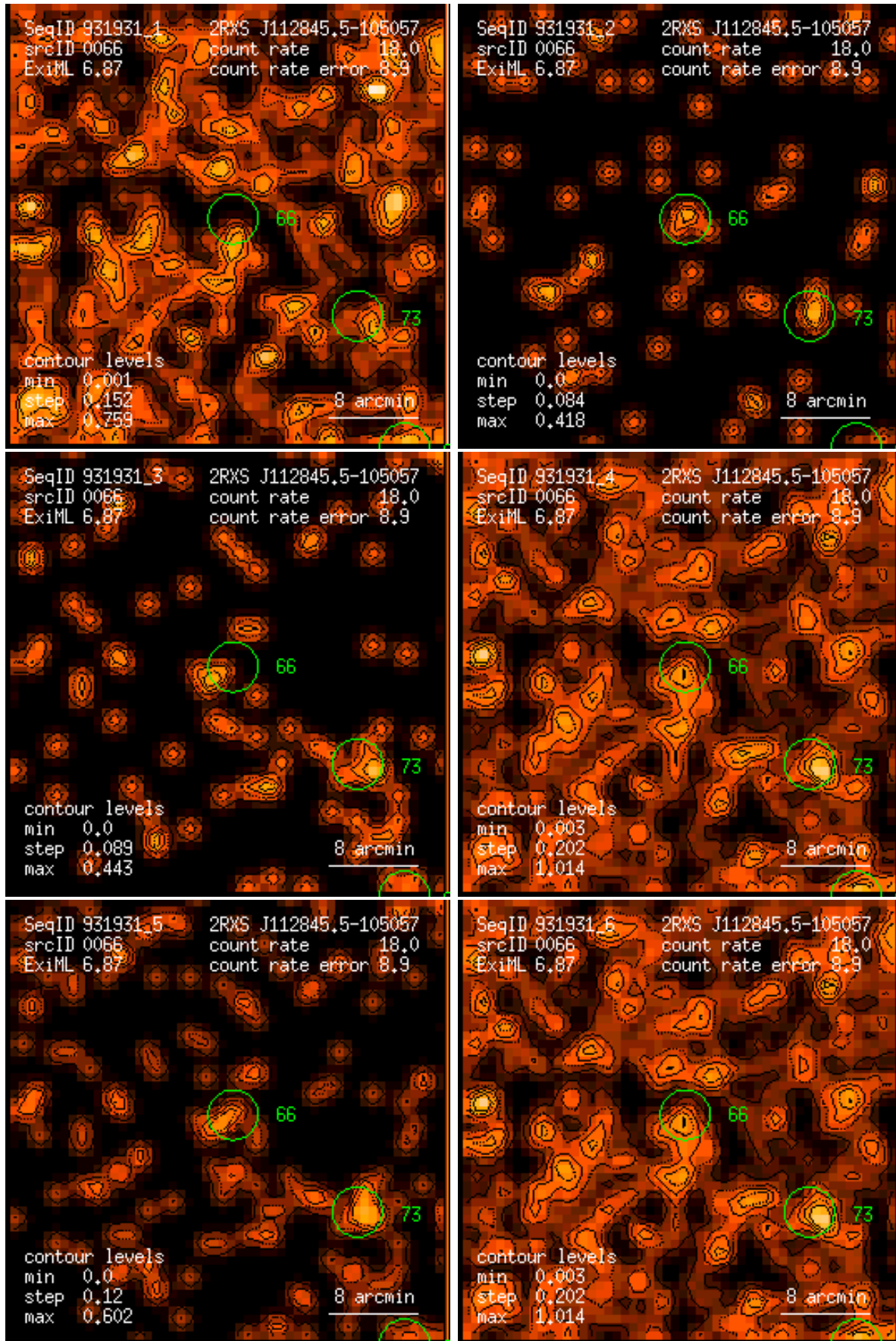
Figure 66: RASS 931931: detection 0066: band rate images, Gaussian filter: (1) PSPC channels 11 – 41, (2) 52 – 90, (3) 91 – 201, (4) 11 – 235, (5) 52 – 201, (6) 11 – 201. Broad band rates in counts/ks. Band rate contour levels in counts/ks/arcmin 2 .
