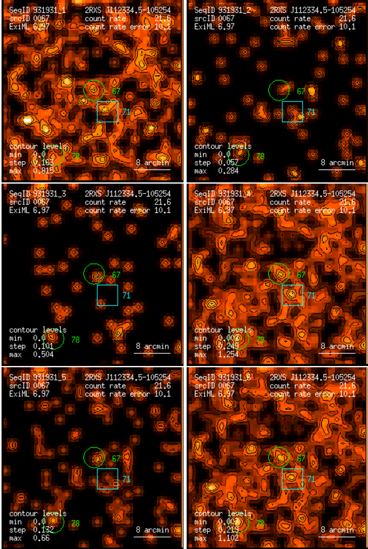
Figure 67: RASS 931931: detection 0067: band rate images, Gaussian filter: (1) PSPC channels 11 – 41, (2) 52 – 90, (3) 91 – 201, (4) 11 – 235, (5) 52 – 201, (6) 11 – 201. Broad band rates in counts/ks. Band rate contour levels in counts/ks/arcmin 2 .
