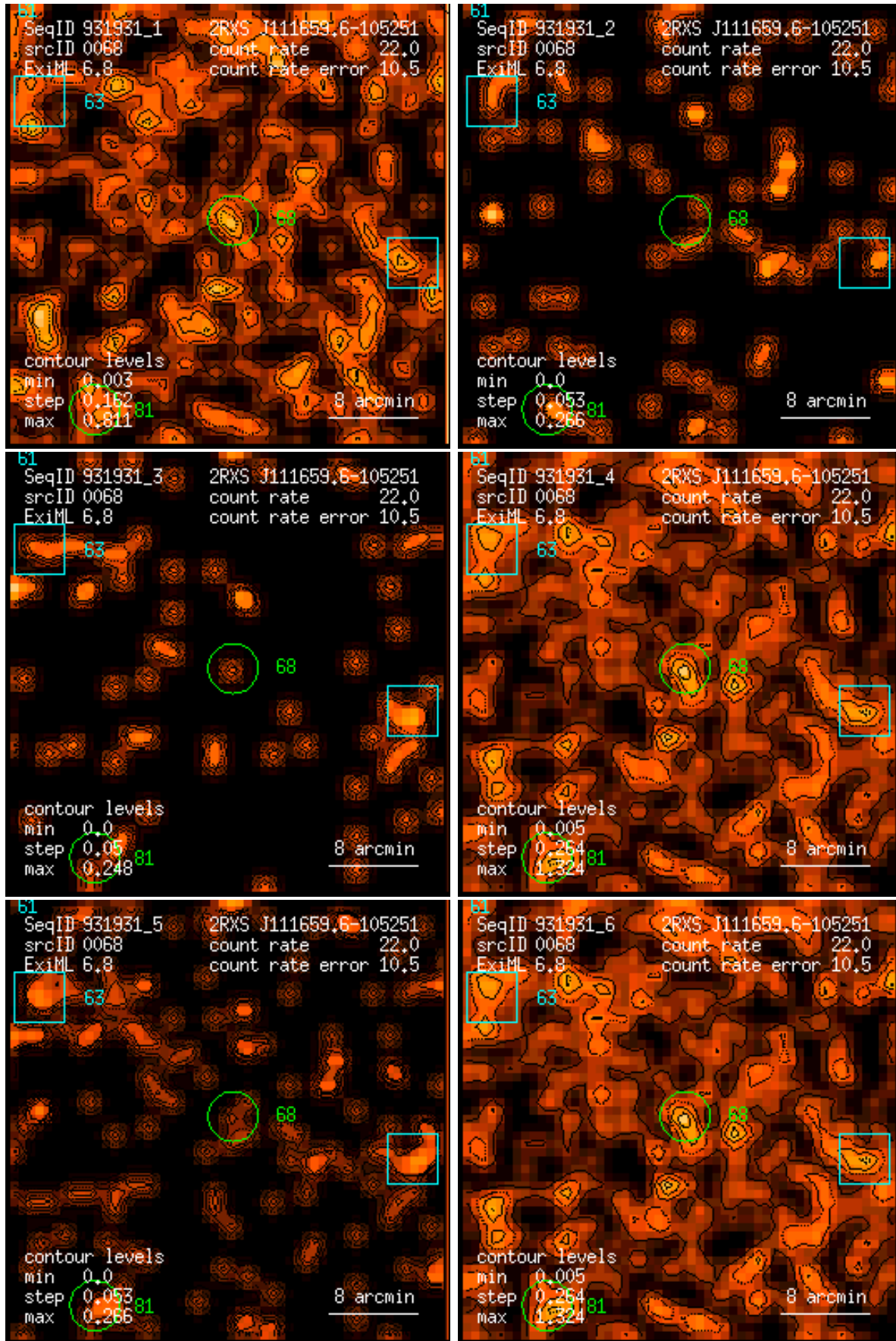
Figure 68: RASS 931931: detection 0068: band rate images, Gaussian filter: (1) PSPC channels 11 – 41, (2) 52 – 90, (3) 91 – 201, (4) 11 – 235, (5) 52 – 201, (6) 11 – 201. Broad band rates in counts/ks. Band rate contour levels in counts/ks/arcmin 2 .
