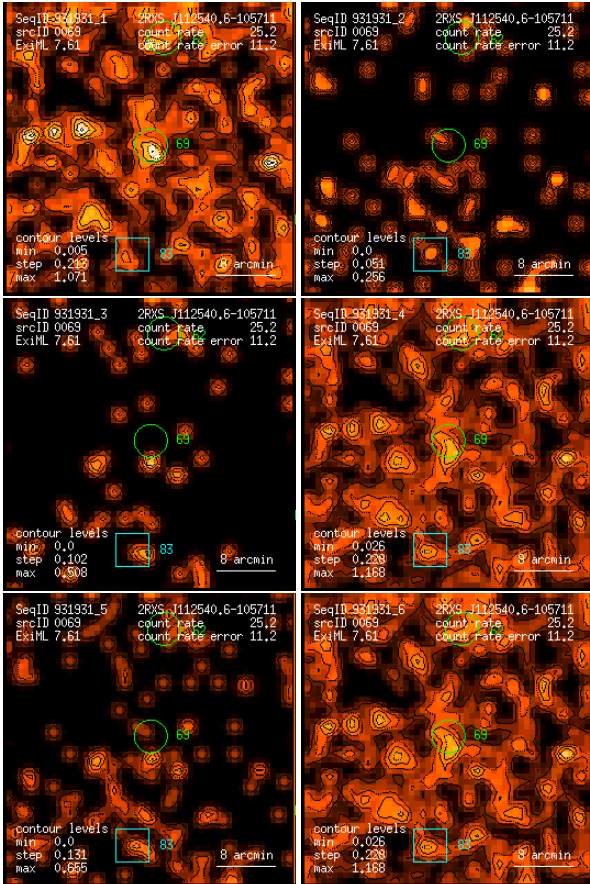
Figure 69: RASS 931931: detection 0069: band rate images, Gaussian filter: (1) PSPC channels 11 – 41, (2) 52 – 90, (3) 91 – 201, (4) 11 – 235, (5) 52 – 201, (6) 11 – 201. Broad band rates in counts/ks. Band rate contour levels in counts/ks/arcmin 2 .
