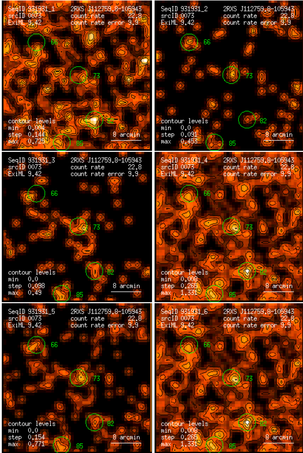
Figure 73: RASS 931931: detection 0073: band rate images, Gaussian filter: (1) PSPC channels 11 – 41, (2) 52 – 90, (3) 91 – 201, (4) 11 – 235, (5) 52 – 201, (6) 11 – 201. Broad band rates in counts/ks. Band rate contour levels in counts/ks/arcmin 2 .
