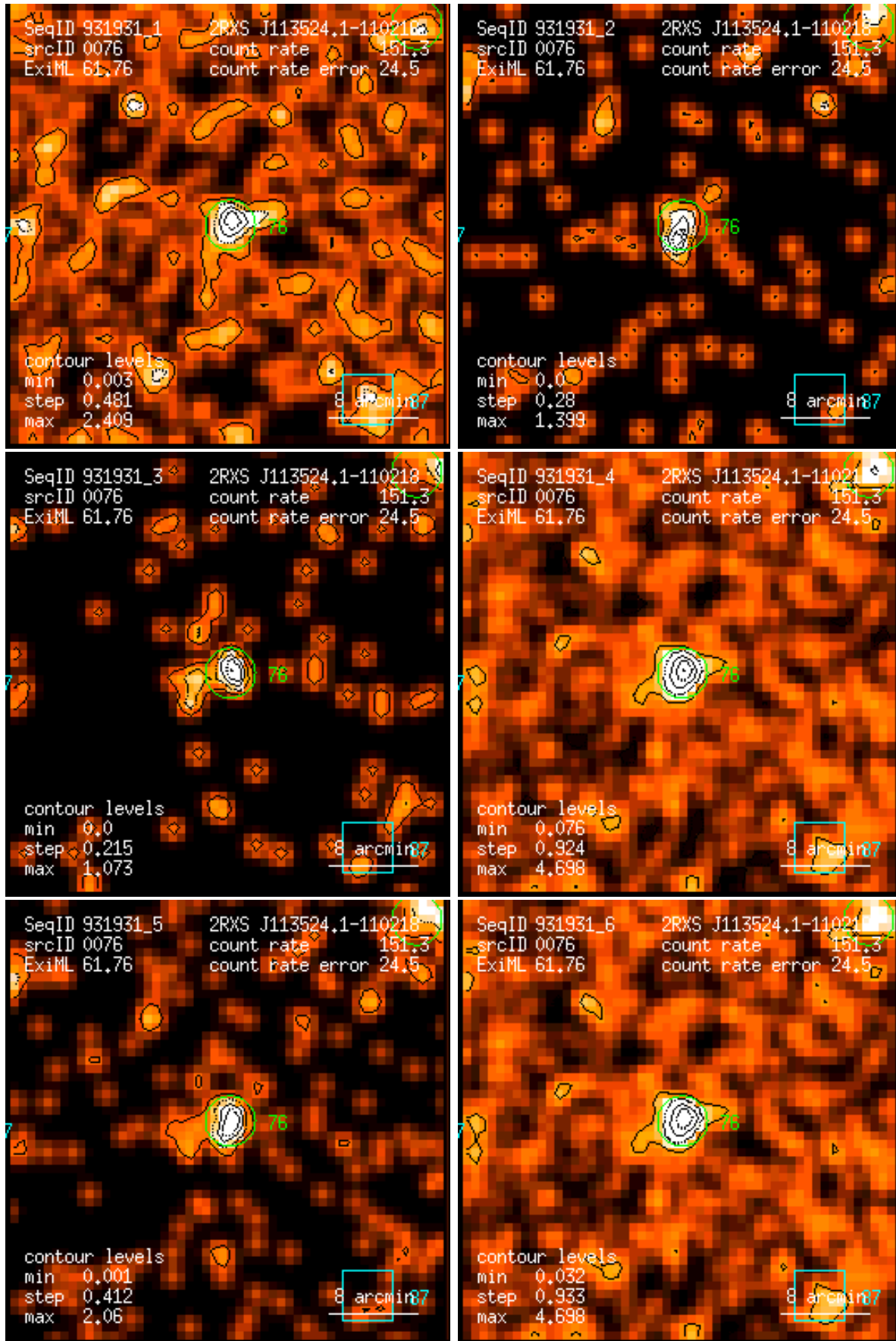
Figure 76: RASS 931931: detection 0076: band rate images, Gaussian filter: (1) PSPC channels 11 – 41, (2) 52 – 90, (3) 91 – 201, (4) 11 – 235, (5) 52 – 201, (6) 11 – 201. Broad band rates in counts/ks. Band rate contour levels in counts/ks/arcmin 2 .
