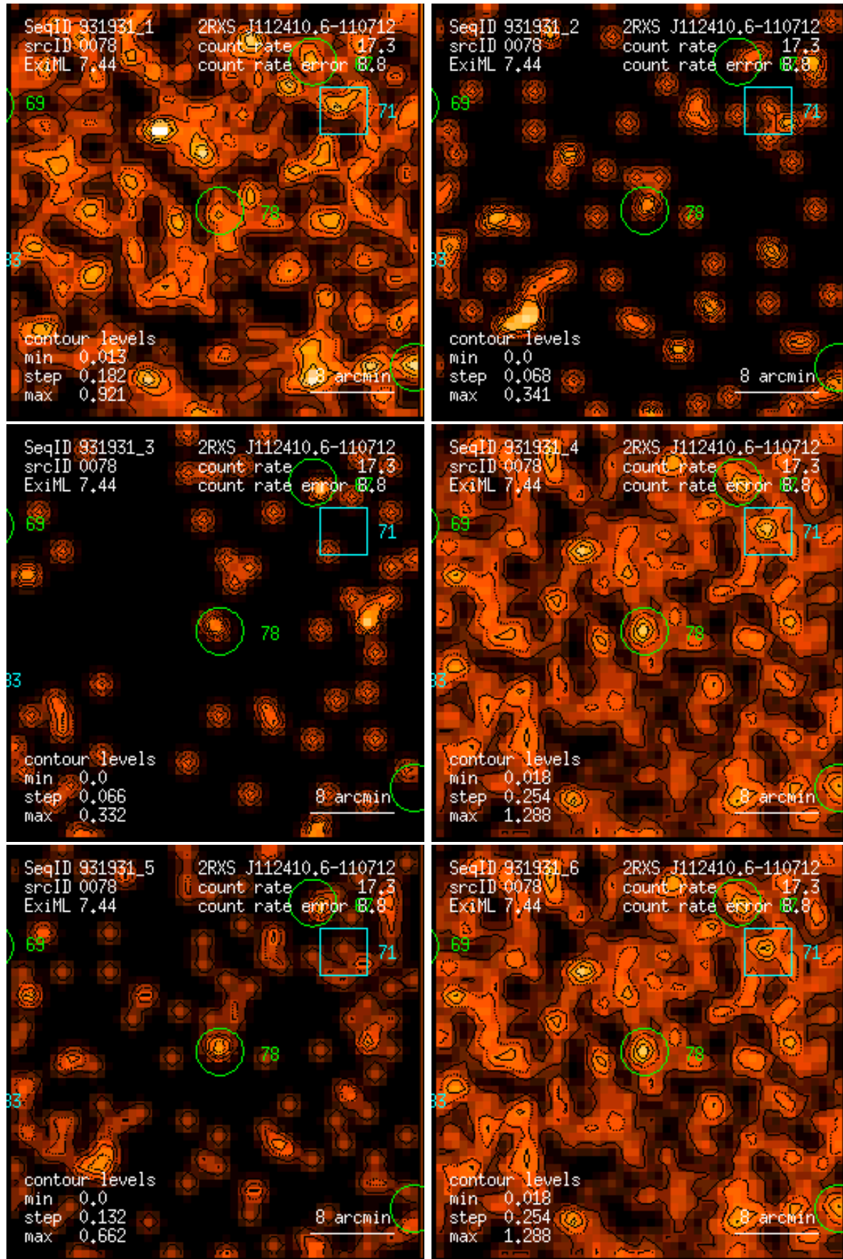
Figure 78: RASS 931931: detection 0078: band rate images, Gaussian filter: (1) PSPC channels 11 – 41, (2) 52 – 90, (3) 91 – 201, (4) 11 – 235, (5) 52 – 201, (6) 11 – 201. Broad band rates in counts/ks. Band rate contour levels in counts/ks/arcmin 2 .
