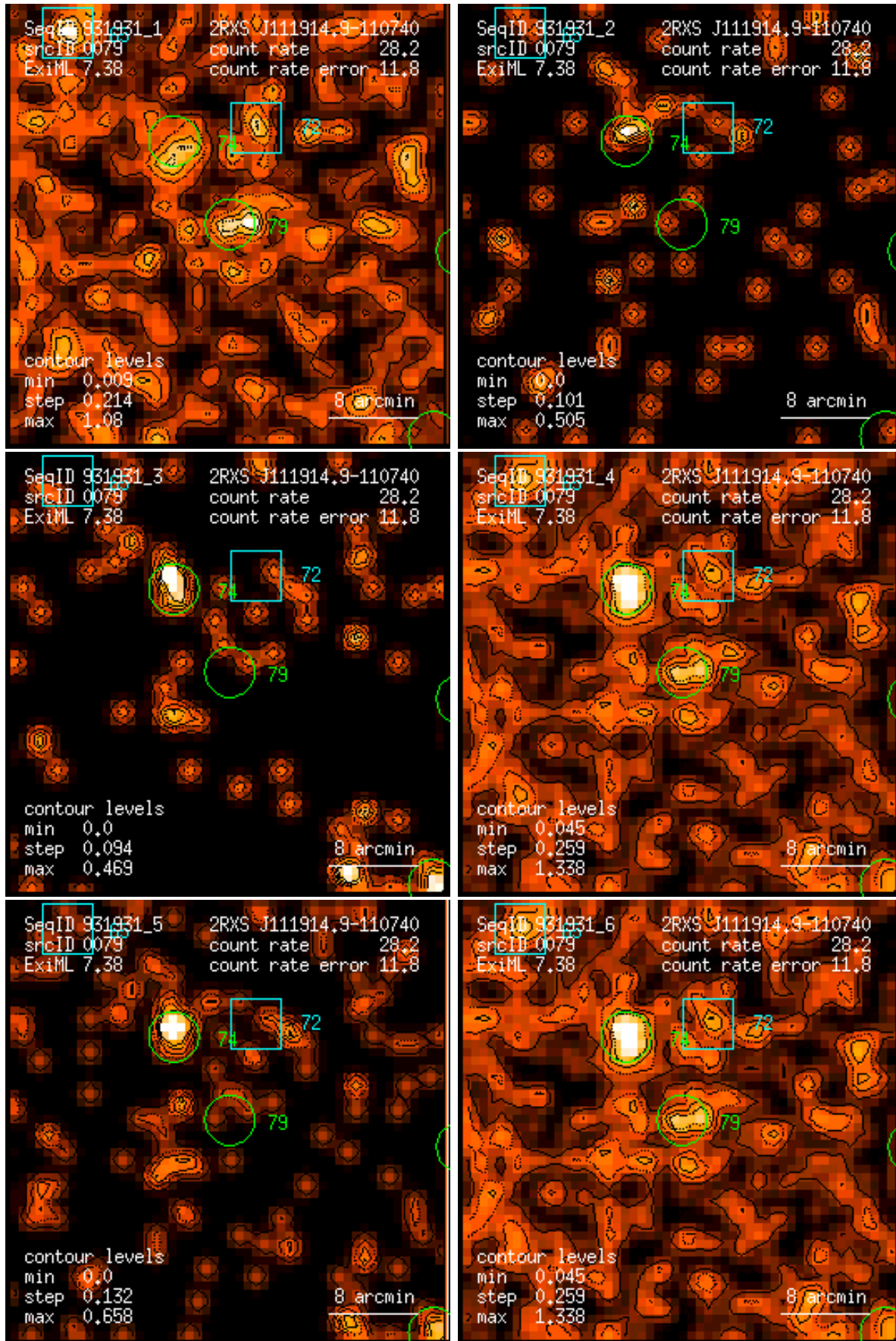
Figure 79: RASS 931931: detection 0079: band rate images, Gaussian filter: (1) PSPC channels 11 – 41, (2) 52 – 90, (3) 91 – 201, (4) 11 – 235, (5) 52 – 201, (6) 11 – 201. Broad band rates in counts/ks. Band rate contour levels in counts/ks/arcmin 2 .
