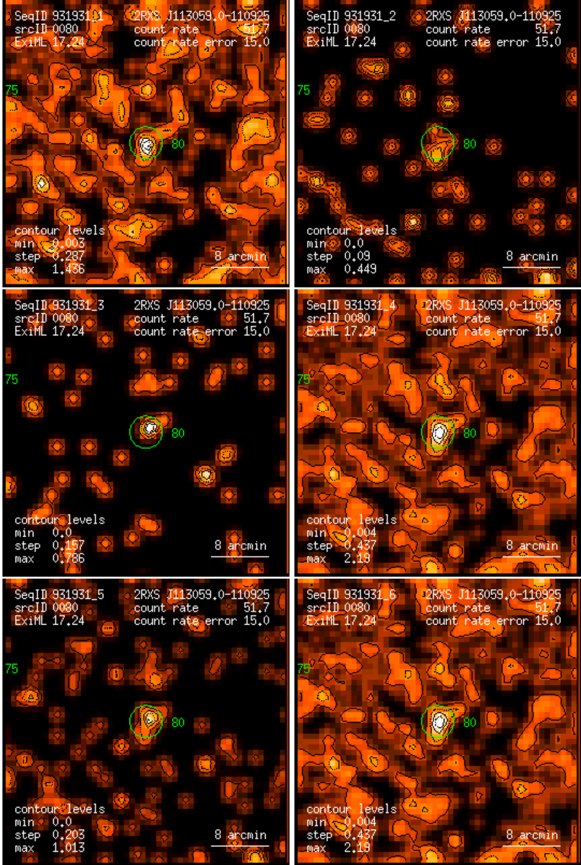
Figure 80: RASS 931931: detection 0080: band rate images, Gaussian filter: (1) PSPC channels 11 – 41, (2) 52 – 90, (3) 91 – 201, (4) 11 – 235, (5) 52 – 201, (6) 11 – 201. Broad band rates in counts/ks. Band rate contour levels in counts/ks/arcmin 2 .
