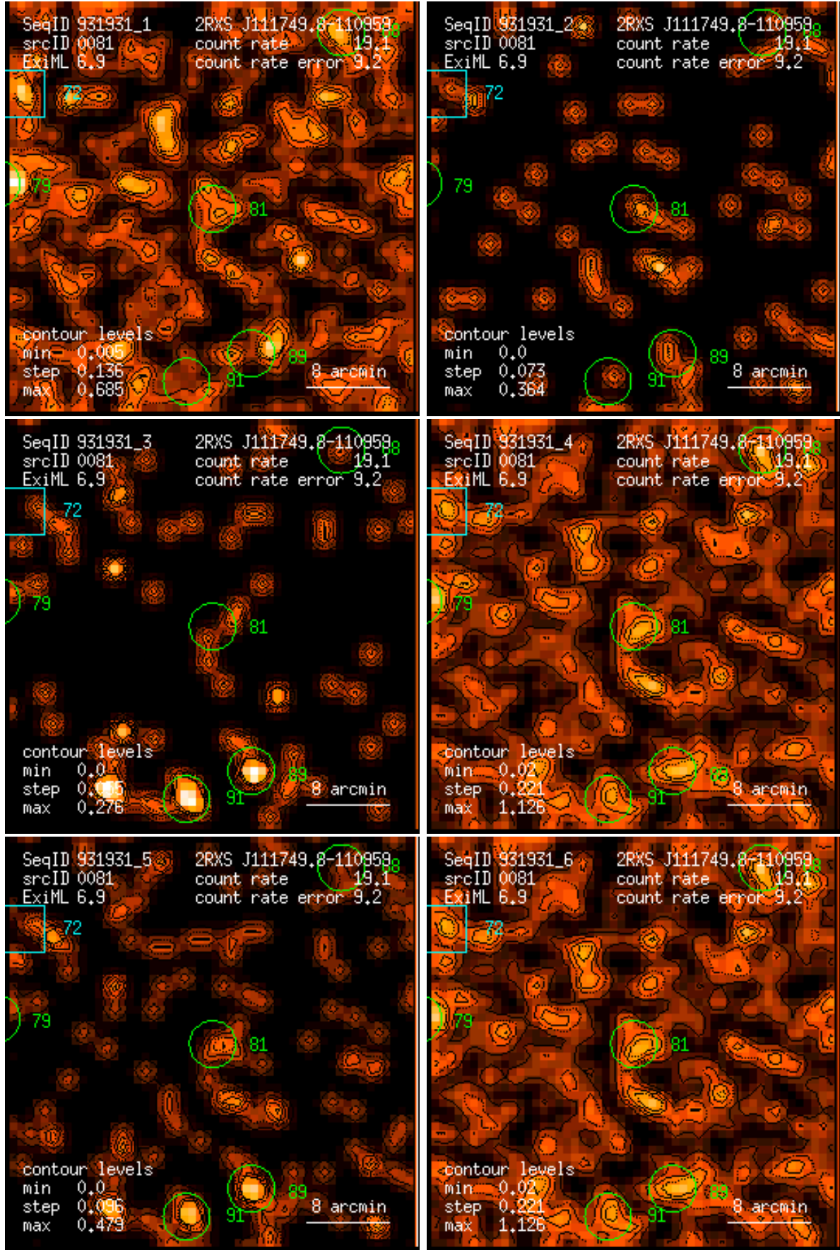
Figure 81: RASS 931931: detection 0081: band rate images, Gaussian filter: (1) PSPC channels 11 – 41, (2) 52 – 90, (3) 91 – 201, (4) 11 – 235, (5) 52 – 201, (6) 11 – 201. Broad band rates in counts/ks. Band rate contour levels in counts/ks/arcmin 2 .
