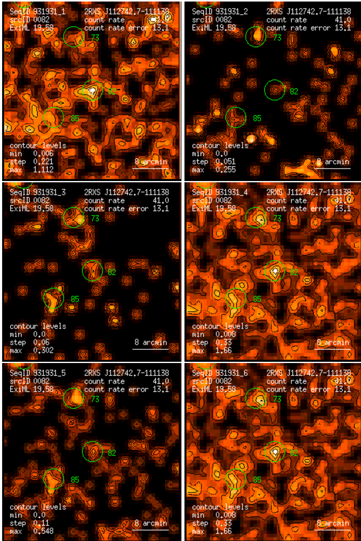
Figure 82: RASS 931931: detection 0082: band rate images, Gaussian filter: (1) PSPC channels 11 – 41, (2) 52 – 90, (3) 91 – 201, (4) 11 – 235, (5) 52 – 201, (6) 11 – 201. Broad band rates in counts/ks. Band rate contour levels in counts/ks/arcmin 2 .
