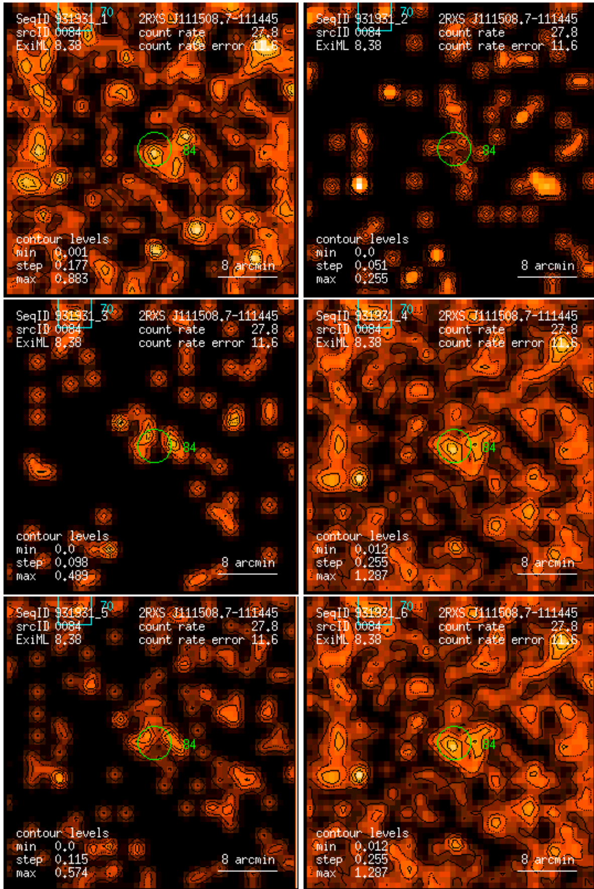
Figure 84: RASS 931931: detection 0084: band rate images, Gaussian filter: (1) PSPC channels 11 – 41, (2) 52 – 90, (3) 91 – 201, (4) 11 – 235, (5) 52 – 201, (6) 11 – 201. Broad band rates in counts/ks. Band rate contour levels in counts/ks/arcmin 2 .
