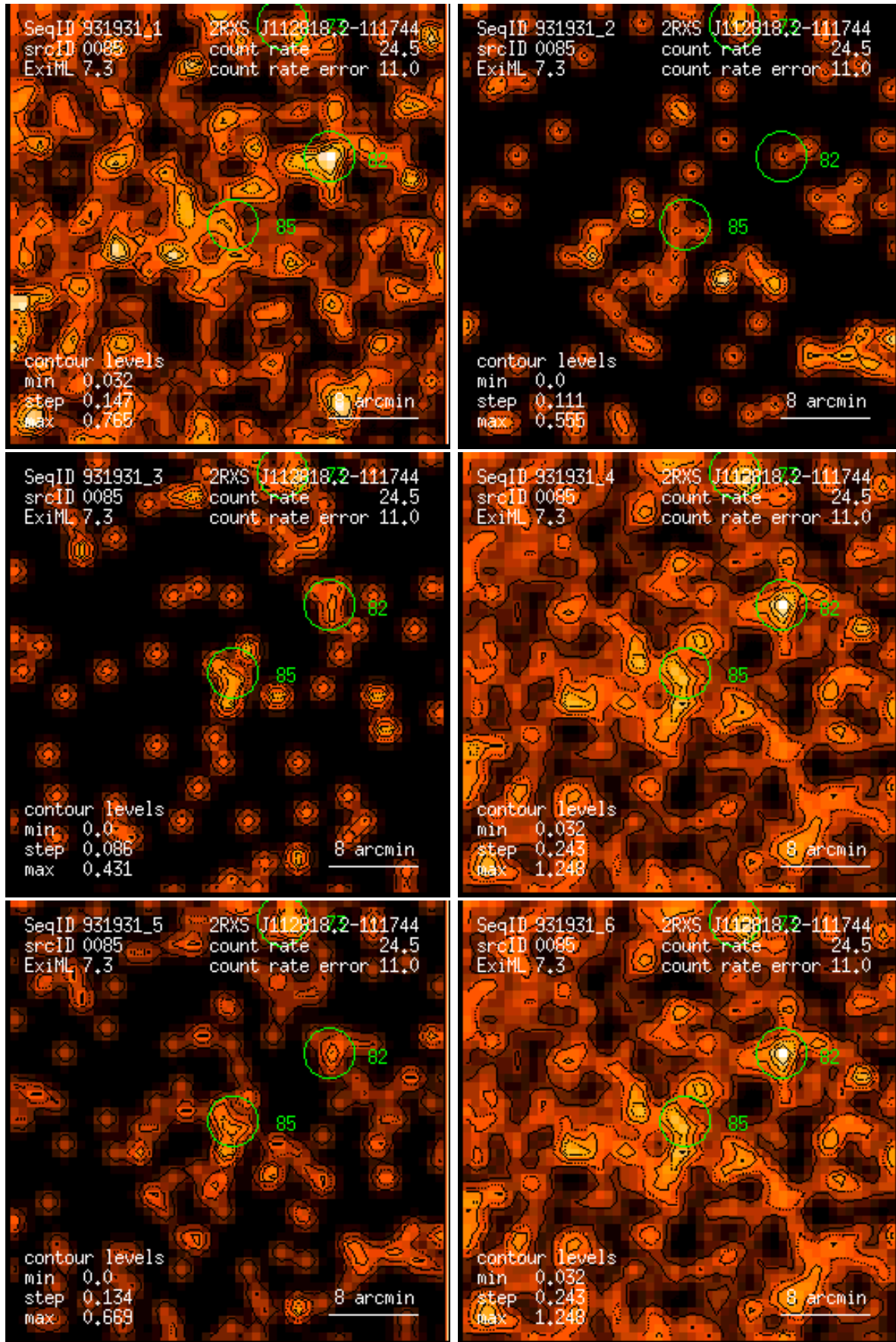
Figure 85: RASS 931931: detection 0085: band rate images, Gaussian filter: (1) PSPC channels 11 – 41, (2) 52 – 90, (3) 91 – 201, (4) 11 – 235, (5) 52 – 201, (6) 11 – 201. Broad band rates in counts/ks. Band rate contour levels in counts/ks/arcmin 2 .
