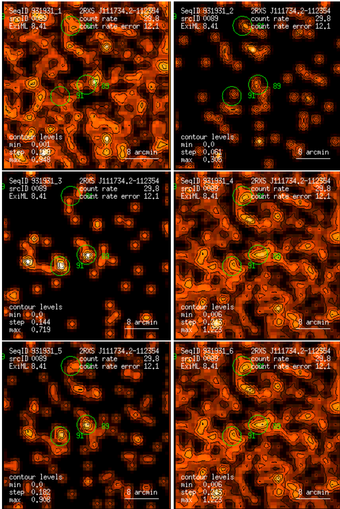
Figure 89: RASS 931931: detection 0089: band rate images, Gaussian filter: (1) PSPC channels 11 – 41, (2) 52 – 90, (3) 91 – 201, (4) 11 – 235, (5) 52 – 201, (6) 11 – 201. Broad band rates in counts/ks. Band rate contour levels in counts/ks/arcmin 2 .
