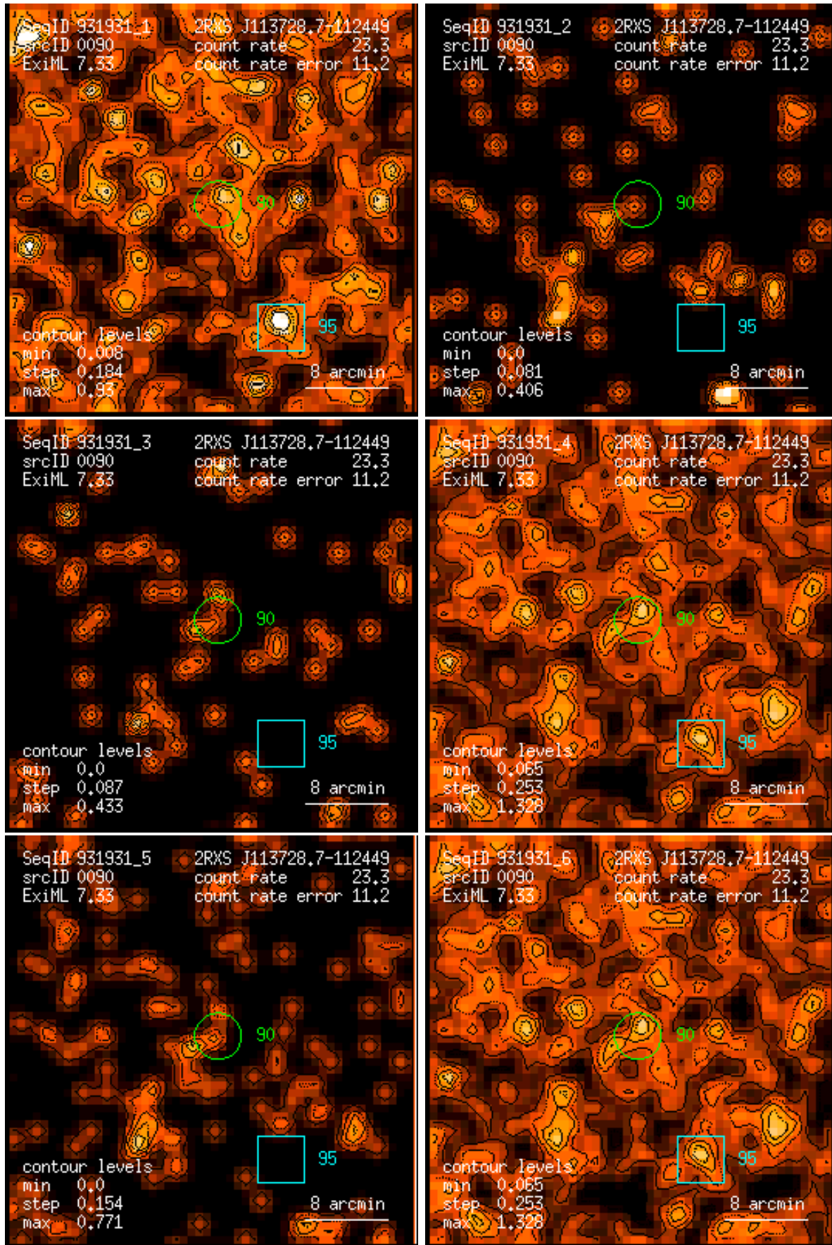
Figure 90: RASS 931931: detection 0090: band rate images, Gaussian filter: (1) PSPC channels 11 – 41, (2) 52 – 90, (3) 91 – 201, (4) 11 – 235, (5) 52 – 201, (6) 11 – 201. Broad band rates in counts/ks. Band rate contour levels in counts/ks/arcmin 2 .
