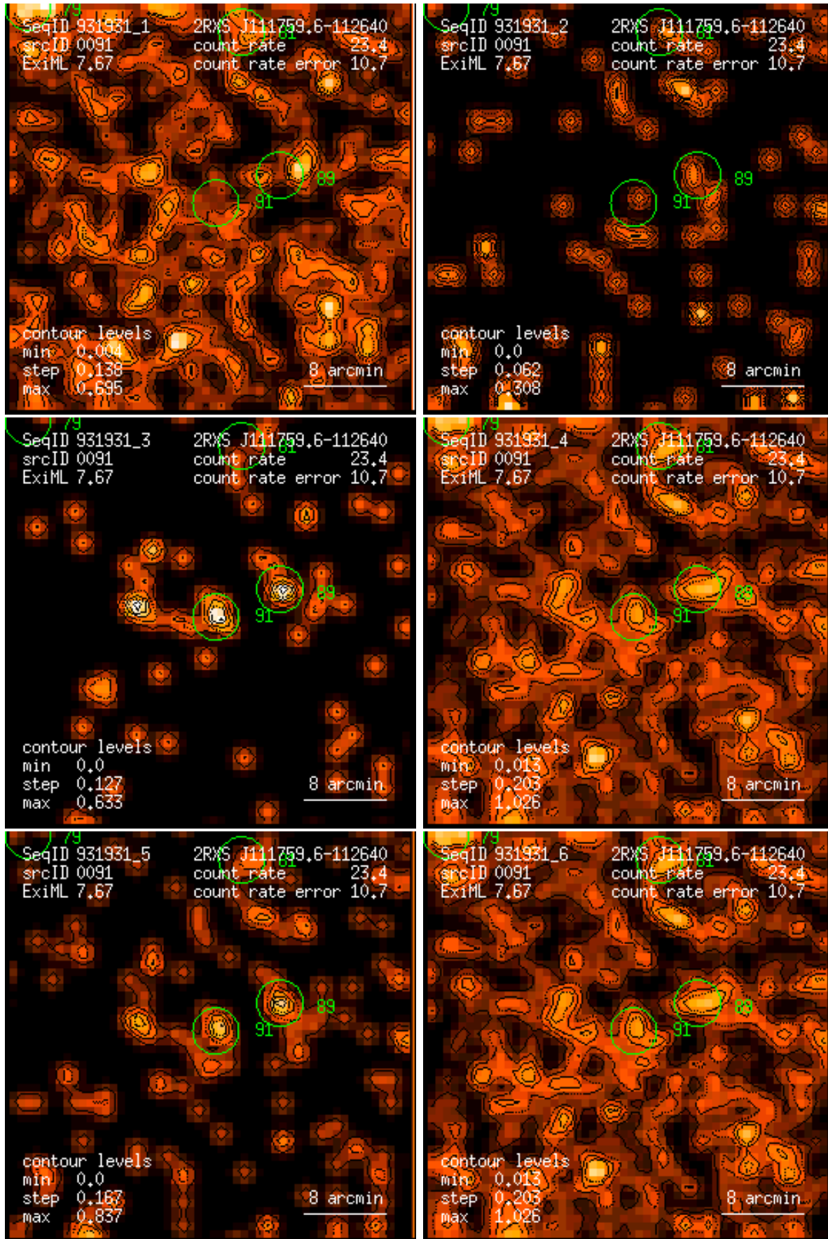
Figure 91: RASS 931931: detection 0091: band rate images, Gaussian filter: (1) PSPC channels 11 – 41, (2) 52 – 90, (3) 91 – 201, (4) 11 – 235, (5) 52 – 201, (6) 11 – 201. Broad band rates in counts/ks. Band rate contour levels in counts/ks/arcmin 2 .
