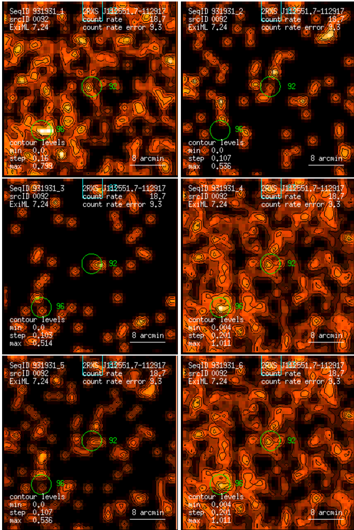
Figure 92: RASS 931931: detection 0092: band rate images, Gaussian filter: (1) PSPC channels 11 – 41, (2) 52 – 90, (3) 91 – 201, (4) 11 – 235, (5) 52 – 201, (6) 11 – 201. Broad band rates in counts/ks. Band rate contour levels in counts/ks/arcmin 2 .
