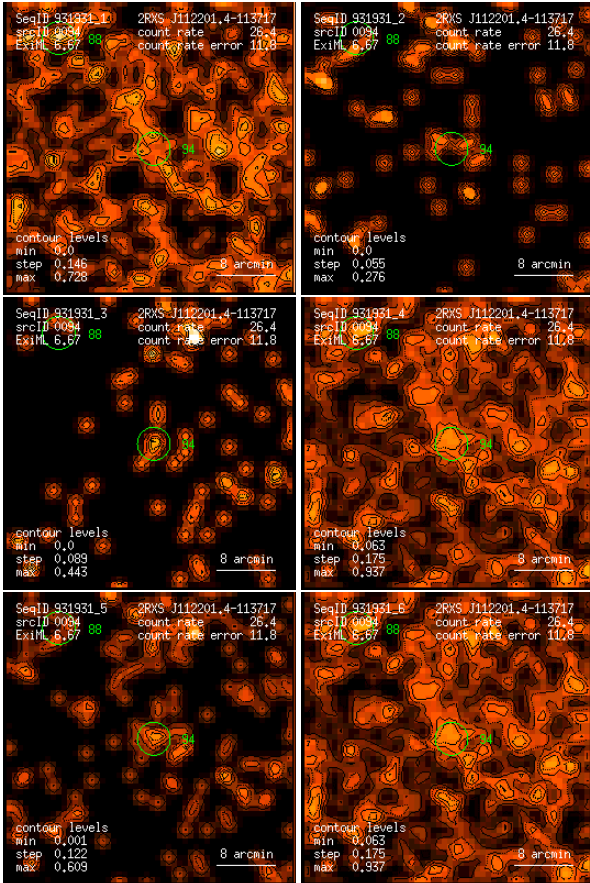
Figure 94: RASS 931931: detection 0094: band rate images, Gaussian filter: (1) PSPC channels 11 – 41, (2) 52 – 90, (3) 91 – 201, (4) 11 – 235, (5) 52 – 201, (6) 11 – 201. Broad band rates in counts/ks. Band rate contour levels in counts/ks/arcmin 2 .
