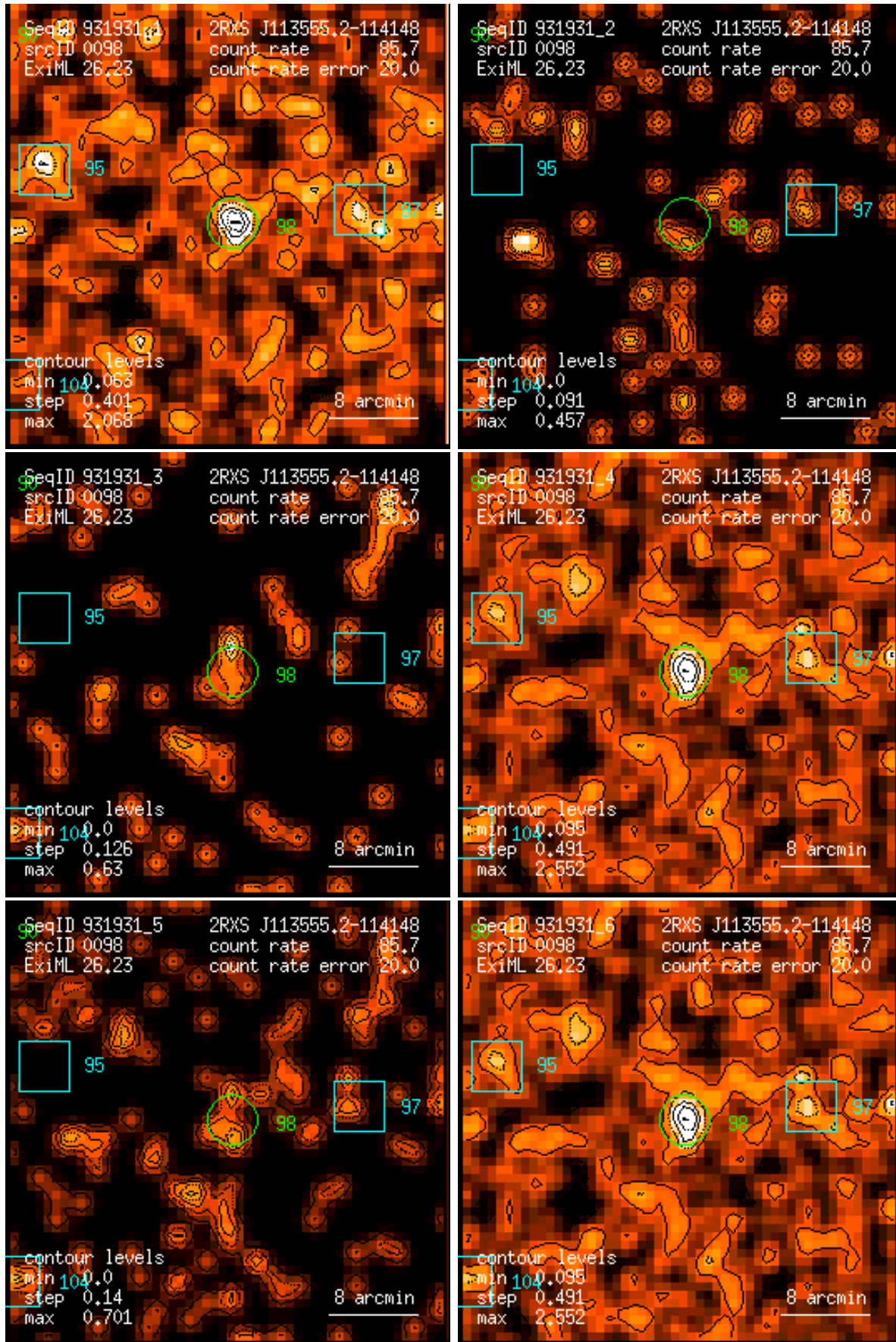
Figure 98: RASS 931931: detection 0098: band rate images, Gaussian filter: (1) PSPC channels 11 – 41, (2) 52 – 90, (3) 91 – 201, (4) 11 – 235, (5) 52 – 201, (6) 11 – 201. Broad band rates in counts/ks. Band rate contour levels in counts/ks/arcmin 2 .
