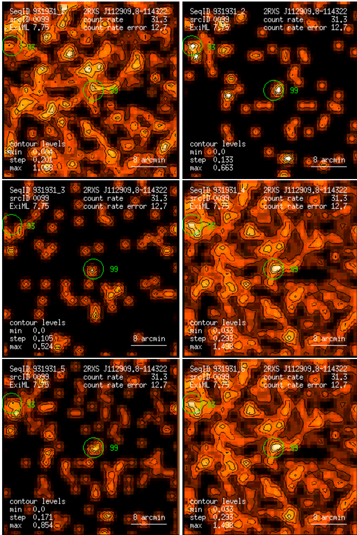
Figure 99: RASS 931931: detection 0099: band rate images, Gaussian filter: (1) PSPC channels 11 – 41, (2) 52 – 90, (3) 91 – 201, (4) 11 – 235, (5) 52 – 201, (6) 11 – 201. Broad band rates in counts/ks. Band rate contour levels in counts/ks/arcmin 2 .
