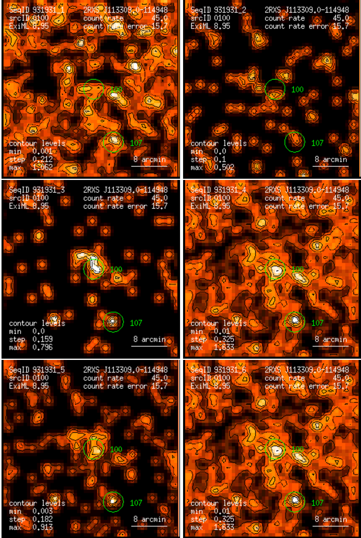
Figure 100: RASS 931931: detection 0100: band rate images, Gaussian filter: (1) PSPC channels 11 – 41, (2) 52 – 90, (3) 91 – 201, (4) 11 – 235, (5) 52 – 201, (6) 11 – 201. Broad band rates in counts/ks. Band rate contour levels in counts/ks/arcmin 2 .
