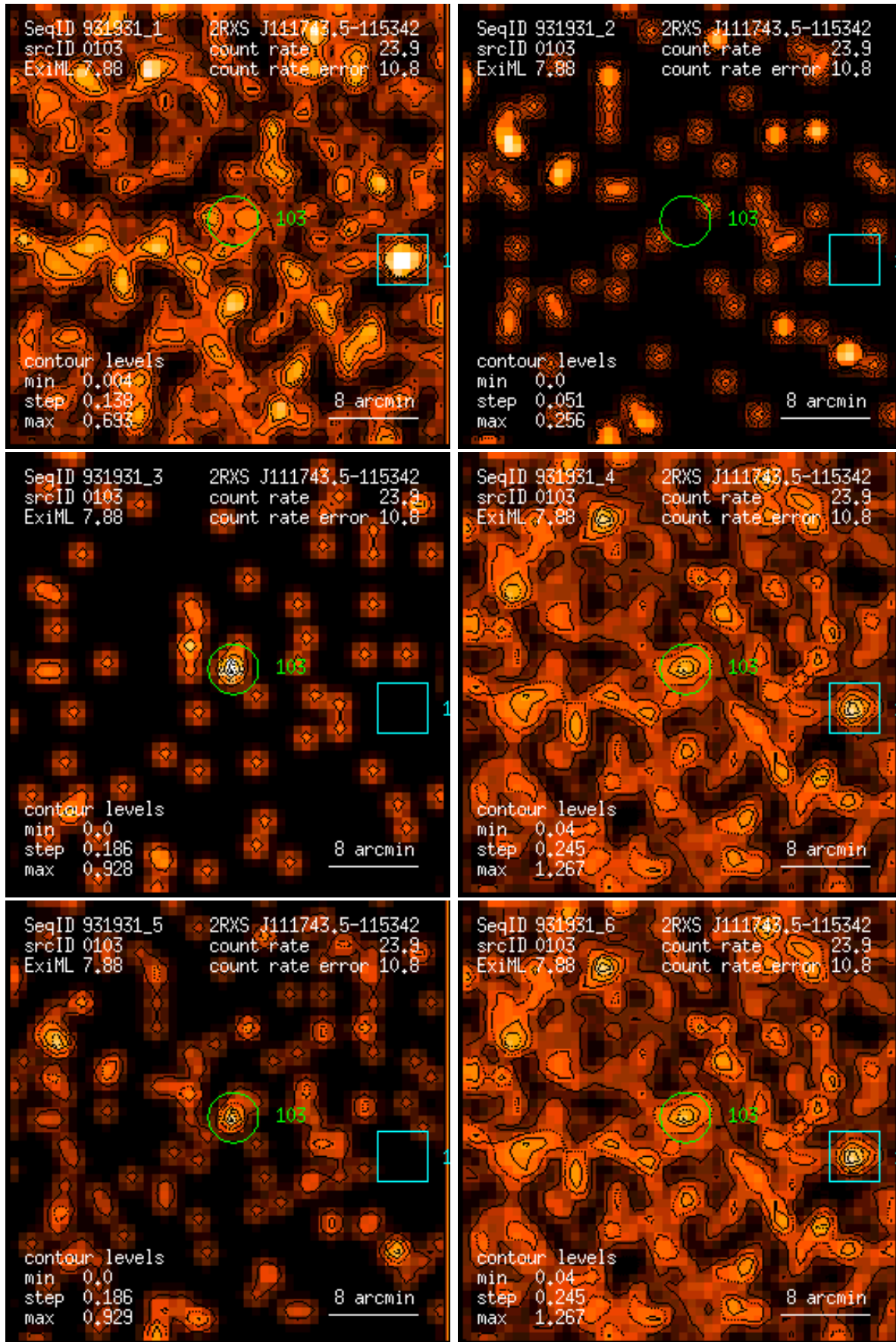
Figure 103: RASS 931931: detection 0103: band rate images, Gaussian filter: (1) PSPC channels 11 – 41, (2) 52 – 90, (3) 91 – 201, (4) 11 – 235, (5) 52 – 201, (6) 11 – 201. Broad band rates in counts/ks. Band rate contour levels in counts/ks/arcmin 2 .
