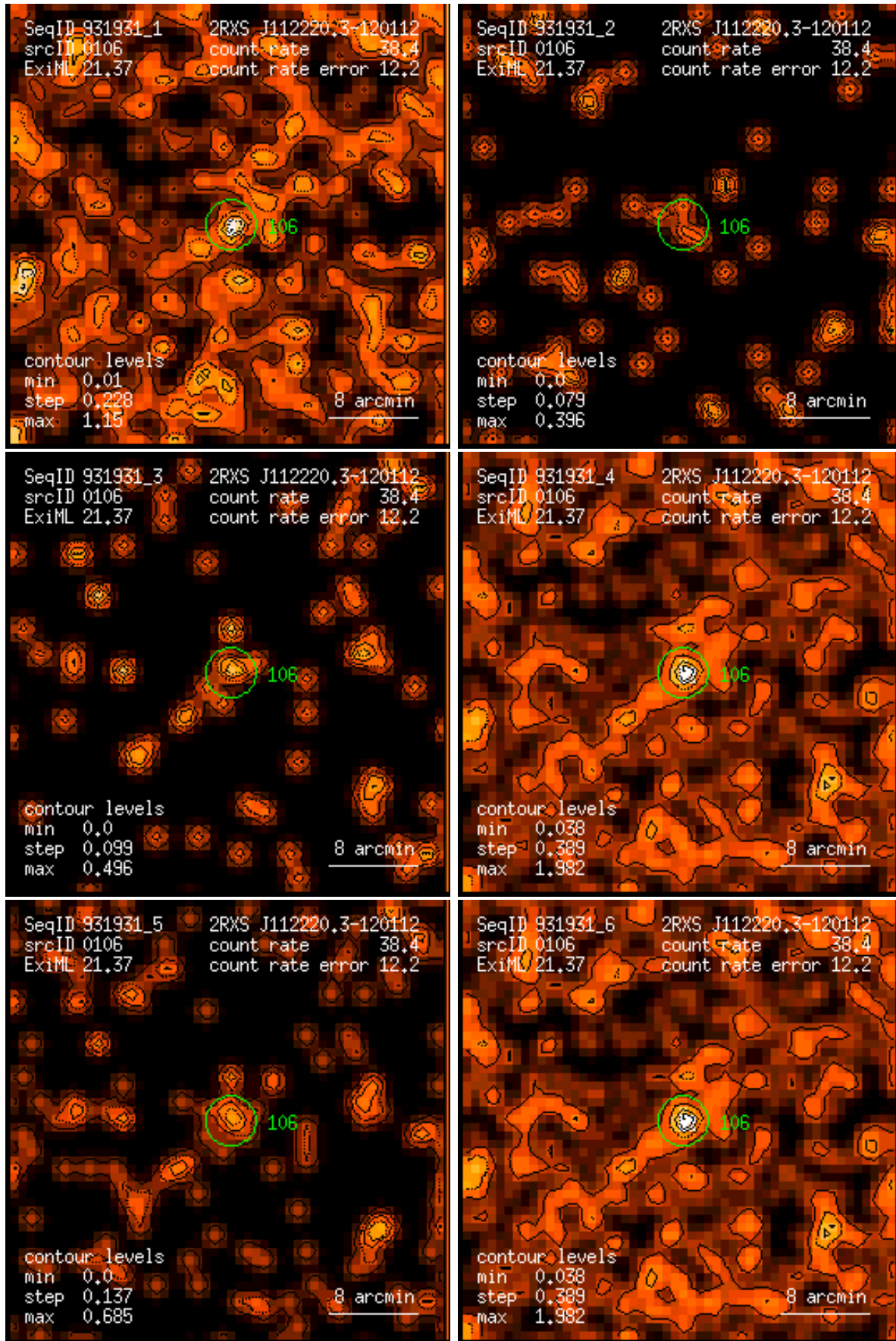
Figure 106: RASS 931931: detection 0106: band rate images, Gaussian filter: (1) PSPC channels 11 – 41, (2) 52 – 90, (3) 91 – 201, (4) 11 – 235, (5) 52 – 201, (6) 11 – 201. Broad band rates in counts/ks. Band rate contour levels in counts/ks/arcmin 2 .
