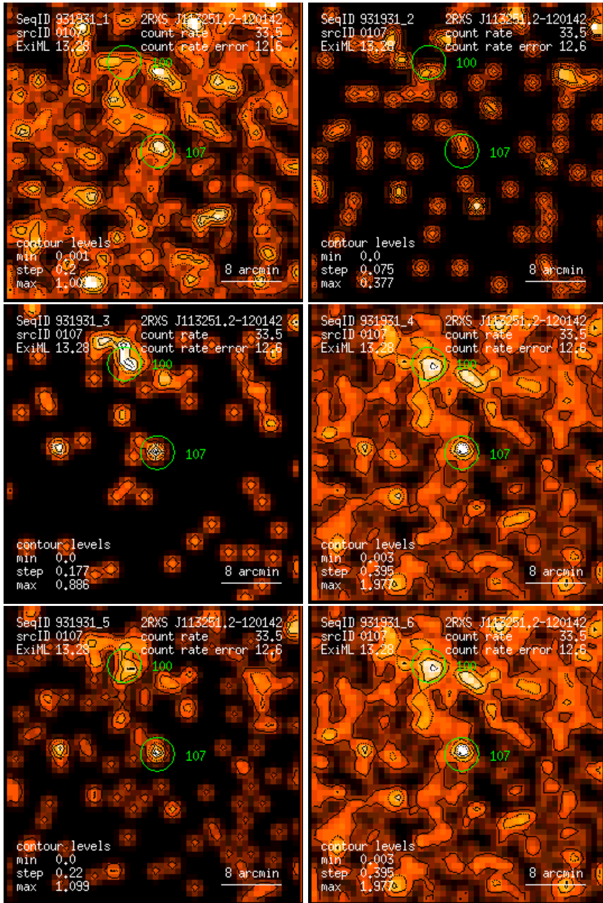
Figure 107: RASS 931931: detection 0107: band rate images, Gaussian filter: (1) PSPC channels 11 – 41, (2) 52 – 90, (3) 91 – 201, (4) 11 – 235, (5) 52 – 201, (6) 11 – 201. Broad band rates in counts/ks. Band rate contour levels in counts/ks/arcmin 2 .
