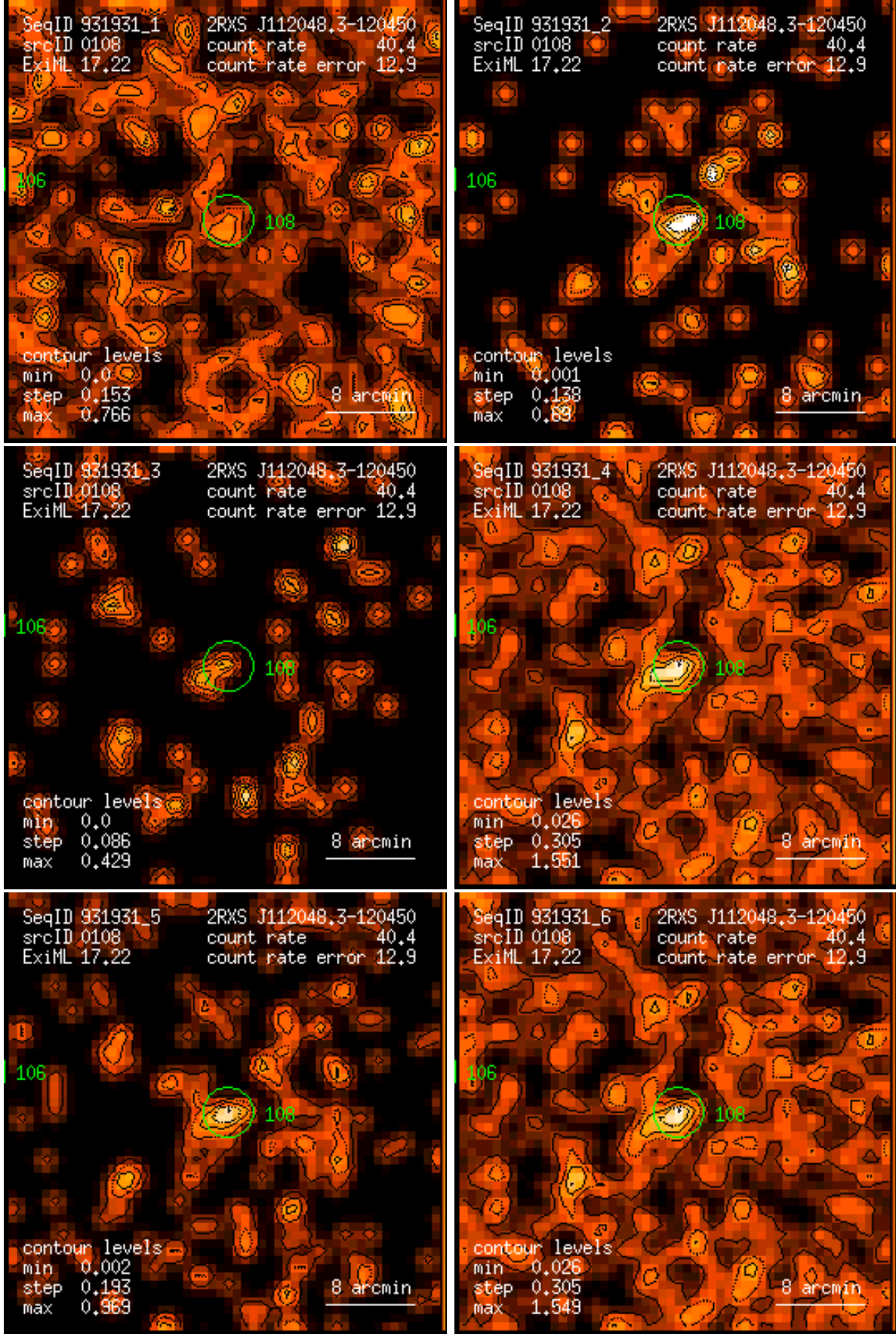
Figure 108: RASS 931931: detection 0108: band rate images, Gaussian filter: (1) PSPC channels 11 – 41, (2) 52 – 90, (3) 91 – 201, (4) 11 – 235, (5) 52 – 201, (6) 11 – 201. Broad band rates in counts/ks. Band rate contour levels in counts/ks/arcmin 2 .
