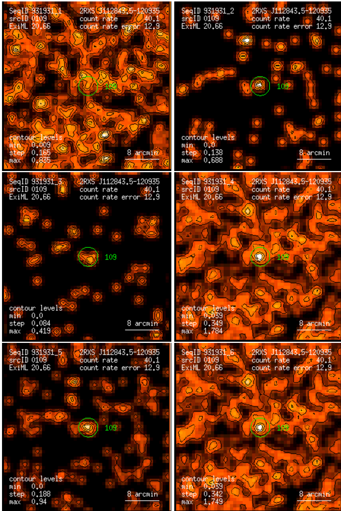
Figure 109: RASS 931931: detection 0109: band rate images, Gaussian filter: (1) PSPC channels 11 – 41, (2) 52 – 90, (3) 91 – 201, (4) 11 – 235, (5) 52 – 201, (6) 11 – 201. Broad band rates in counts/ks. Band rate contour levels in counts/ks/arcmin 2 .
