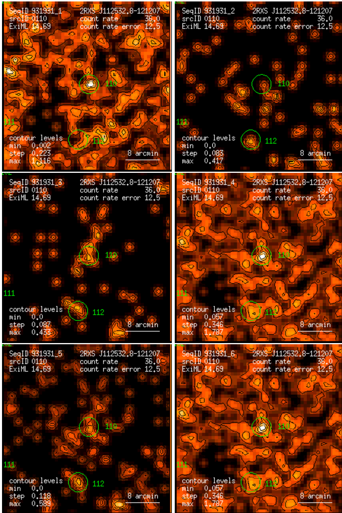
Figure 110: RASS 931931: detection 0110: band rate images, Gaussian filter: (1) PSPC channels 11 – 41, (2) 52 – 90, (3) 91 – 201, (4) 11 – 235, (5) 52 – 201, (6) 11 – 201. Broad band rates in counts/ks. Band rate contour levels in counts/ks/arcmin 2 .
