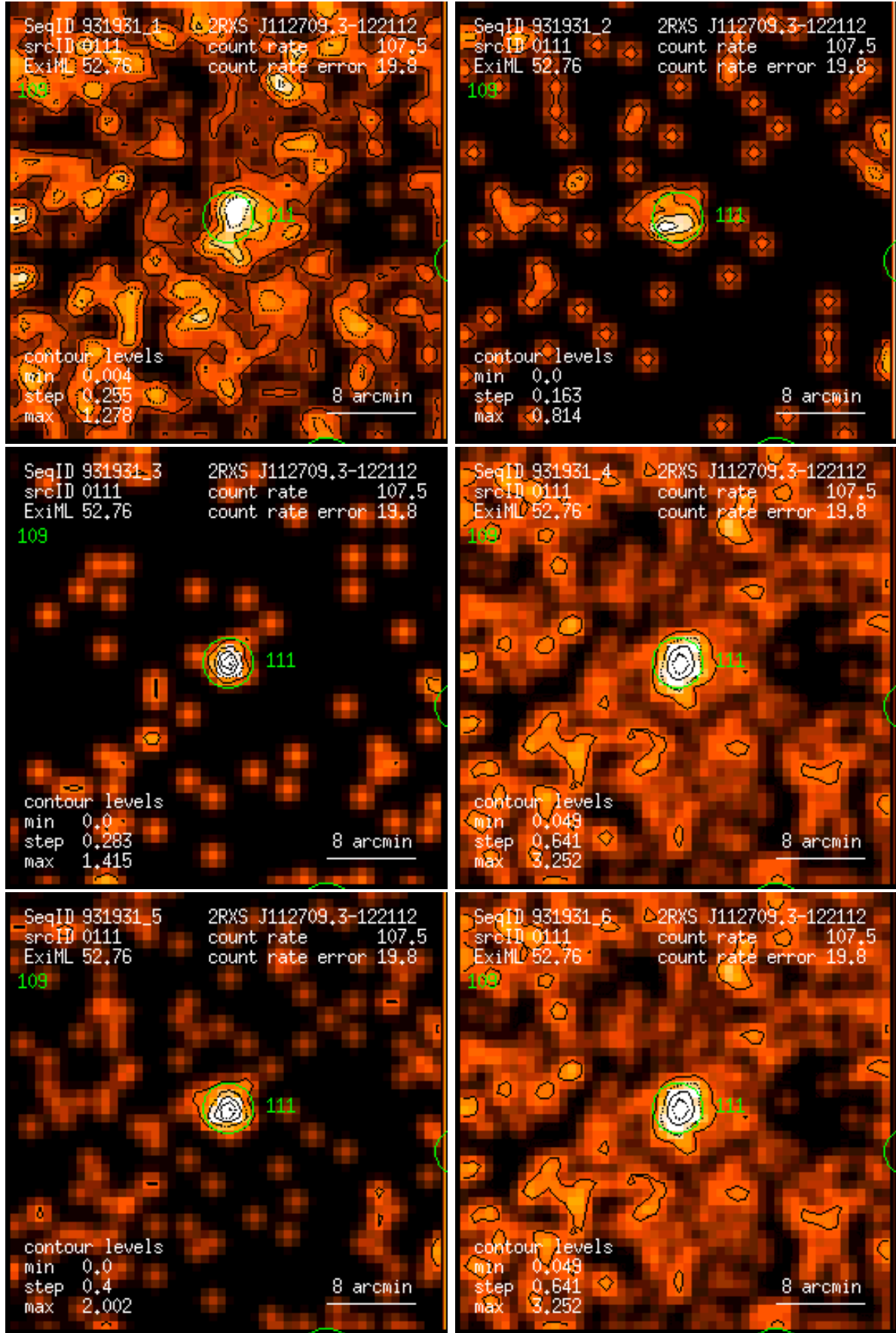
Figure 111: RASS 931931: detection 0111: band rate images, Gaussian filter: (1) PSPC channels 11 – 41, (2) 52 – 90, (3) 91 – 201, (4) 11 – 235, (5) 52 – 201, (6) 11 – 201. Broad band rates in counts/ks. Band rate contour levels in counts/ks/arcmin 2 .
