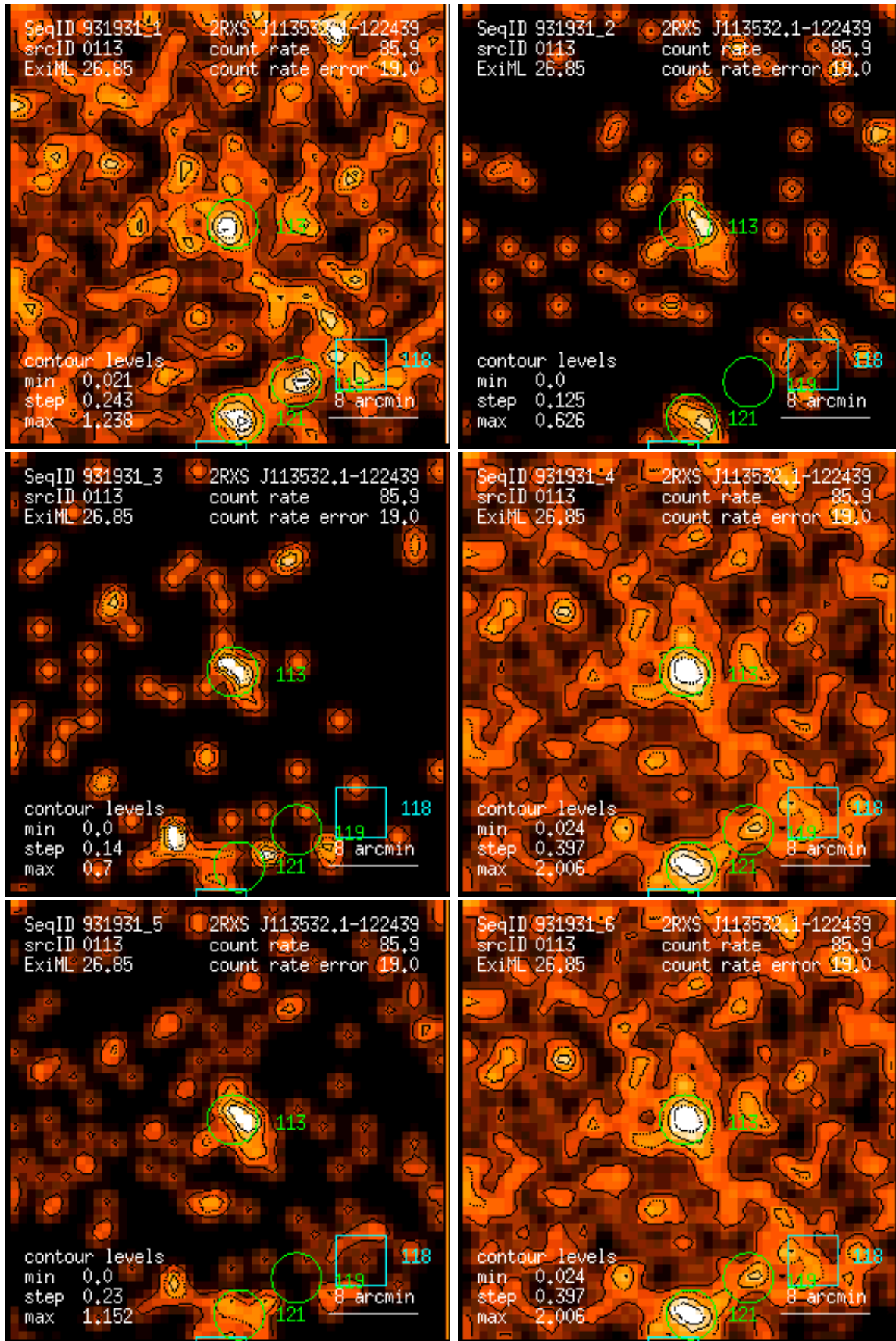
Figure 113: RASS 931931: detection 0113: band rate images, Gaussian filter: (1) PSPC channels 11 – 41, (2) 52 – 90, (3) 91 – 201, (4) 11 – 235, (5) 52 – 201, (6) 11 – 201. Broad band rates in counts/ks. Band rate contour levels in counts/ks/arcmin 2 .
