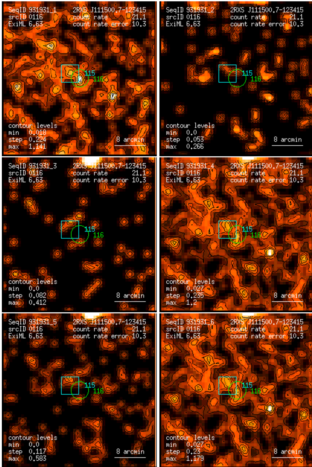
Figure 116: RASS 931931: detection 0116: band rate images, Gaussian filter: (1) PSPC channels 11 – 41, (2) 52 – 90, (3) 91 – 201, (4) 11 – 235, (5) 52 – 201, (6) 11 – 201. Broad band rates in counts/ks. Band rate contour levels in counts/ks/arcmin 2 .
