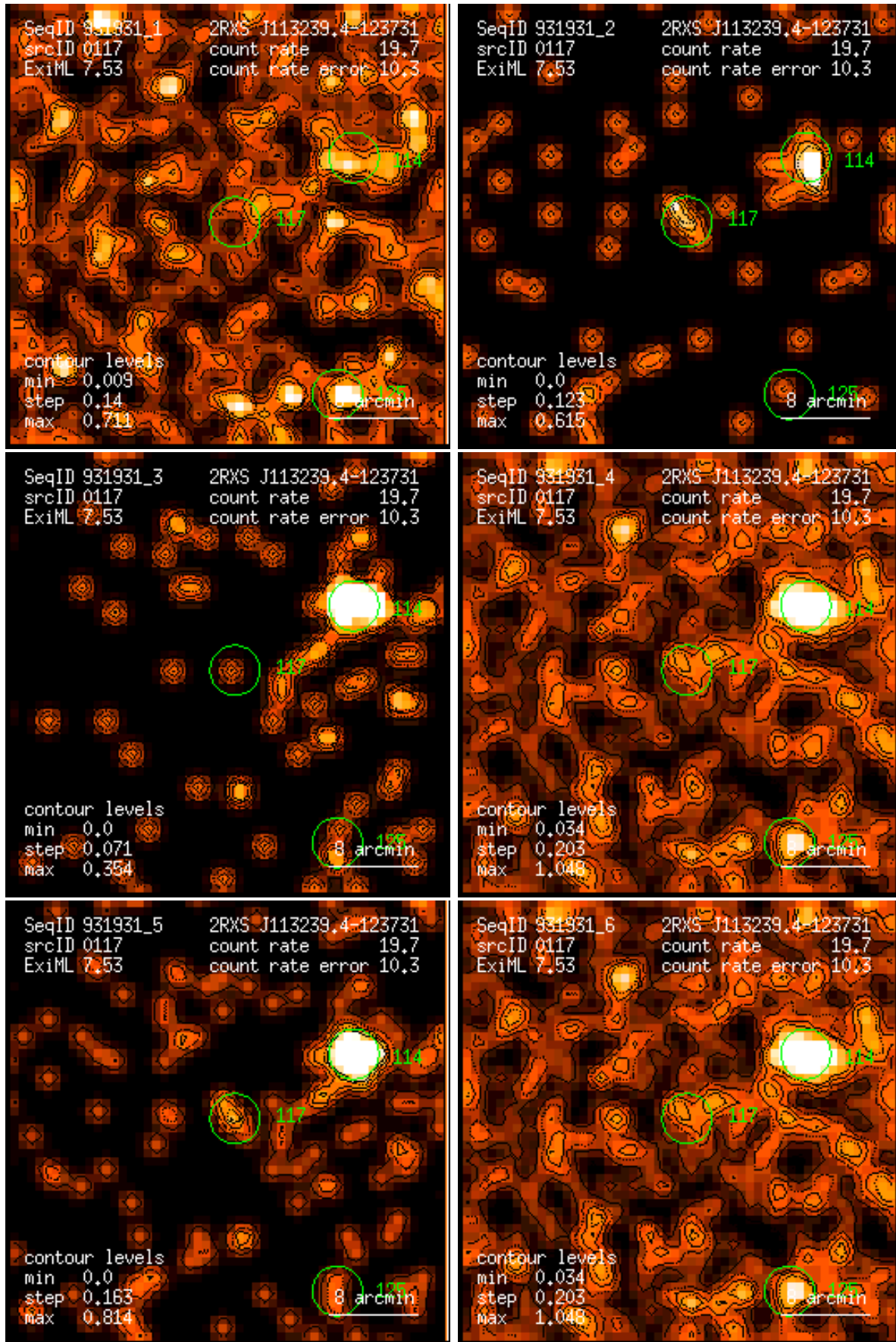
Figure 117: RASS 931931: detection 0117: band rate images, Gaussian filter: (1) PSPC channels 11 – 41, (2) 52 – 90, (3) 91 – 201, (4) 11 – 235, (5) 52 – 201, (6) 11 – 201. Broad band rates in counts/ks. Band rate contour levels in counts/ks/arcmin 2 .
