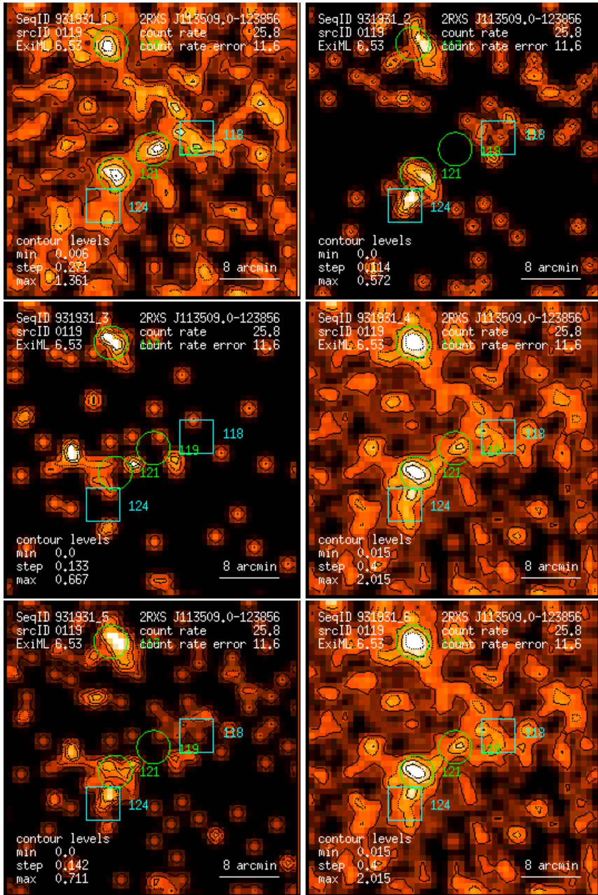
Figure 119: RASS 931931: detection 0119: band rate images, Gaussian filter: (1) PSPC channels 11 – 41, (2) 52 – 90, (3) 91 – 201, (4) 11 – 235, (5) 52 – 201, (6) 11 – 201. Broad band rates in counts/ks. Band rate contour levels in counts/ks/arcmin 2 .
