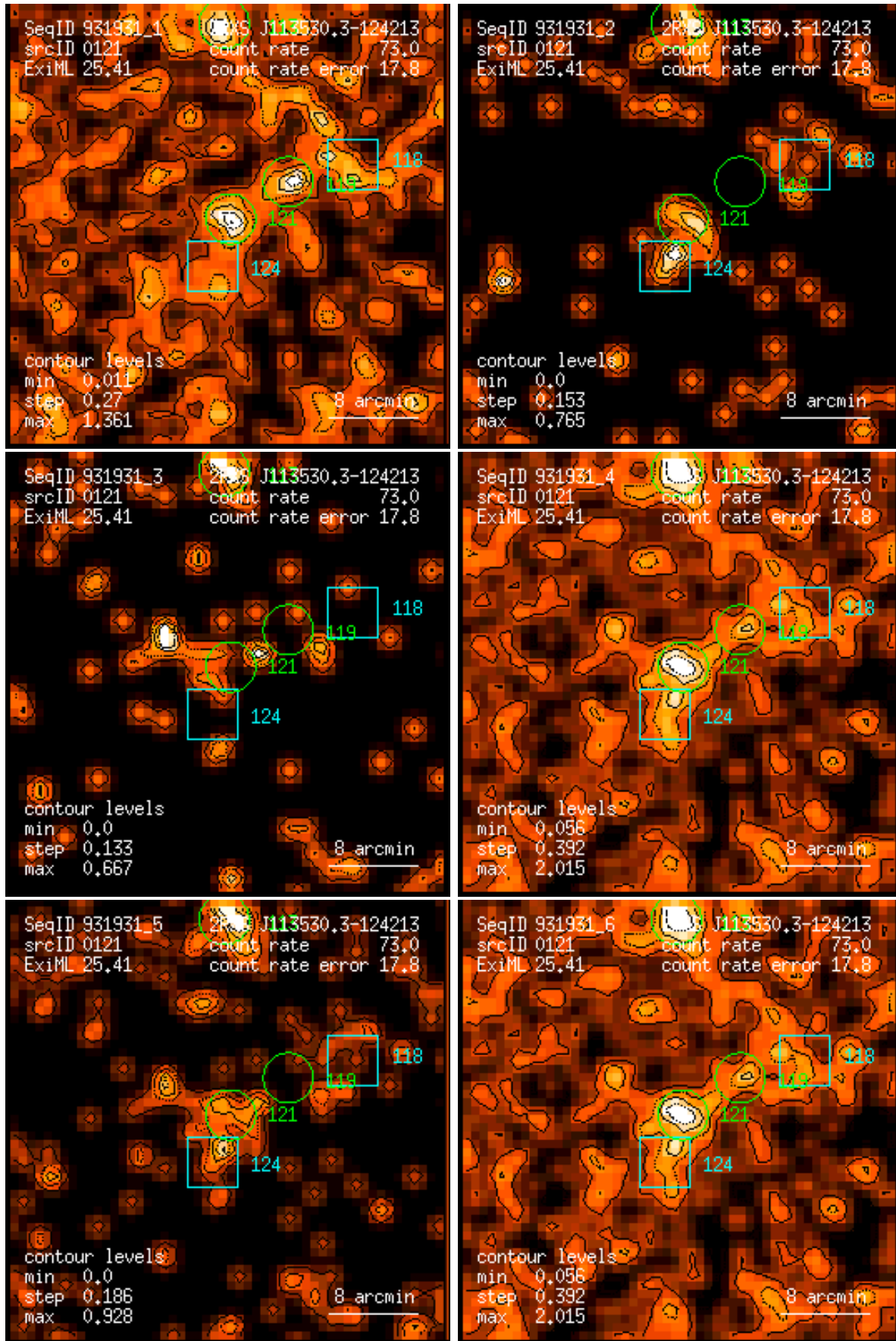
Figure 121: RASS 931931: detection 0121: band rate images, Gaussian filter: (1) PSPC channels 11 – 41, (2) 52 – 90, (3) 91 – 201, (4) 11 – 235, (5) 52 – 201, (6) 11 – 201. Broad band rates in counts/ks. Band rate contour levels in counts/ks/arcmin 2 .
