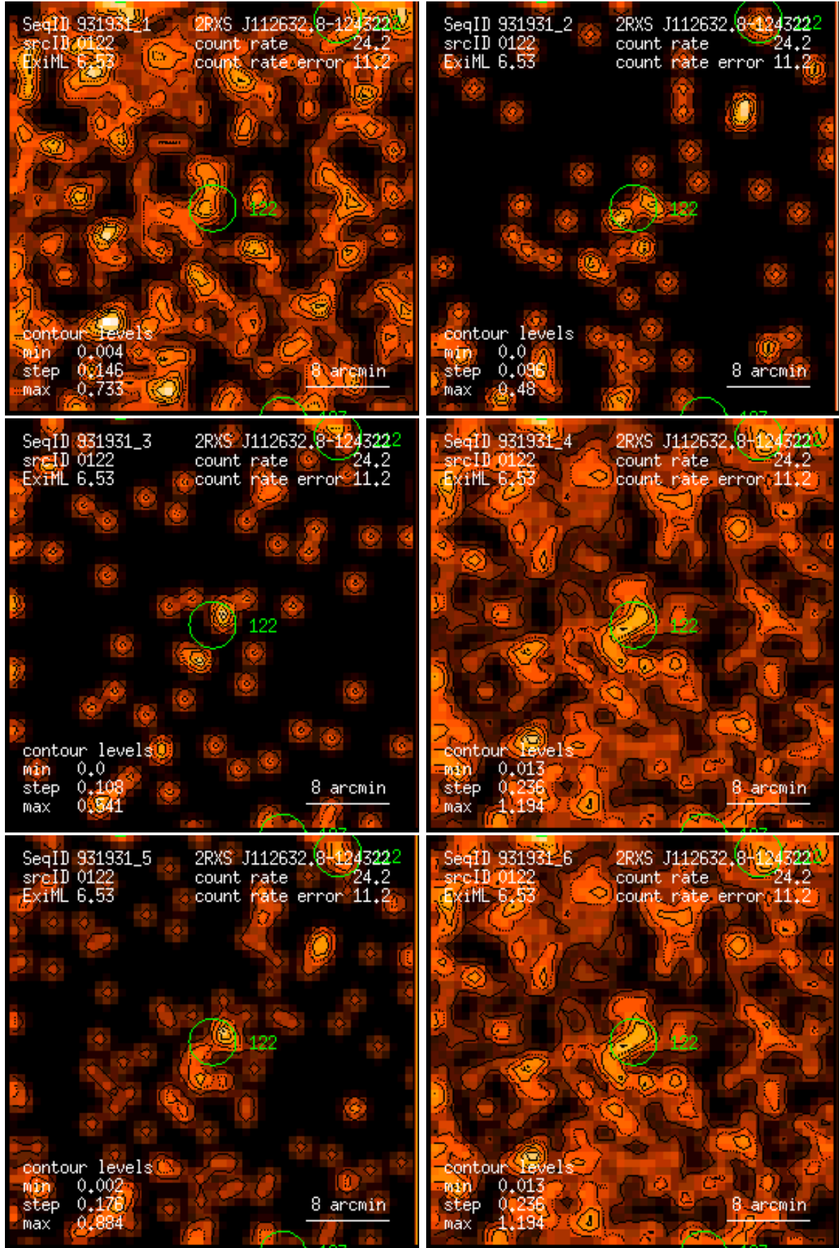
Figure 122: RASS 931931: detection 0122: band rate images, Gaussian filter: (1) PSPC channels 11 – 41, (2) 52 – 90, (3) 91 – 201, (4) 11 – 235, (5) 52 – 201, (6) 11 – 201. Broad band rates in counts/ks. Band rate contour levels in counts/ks/arcmin 2 .
