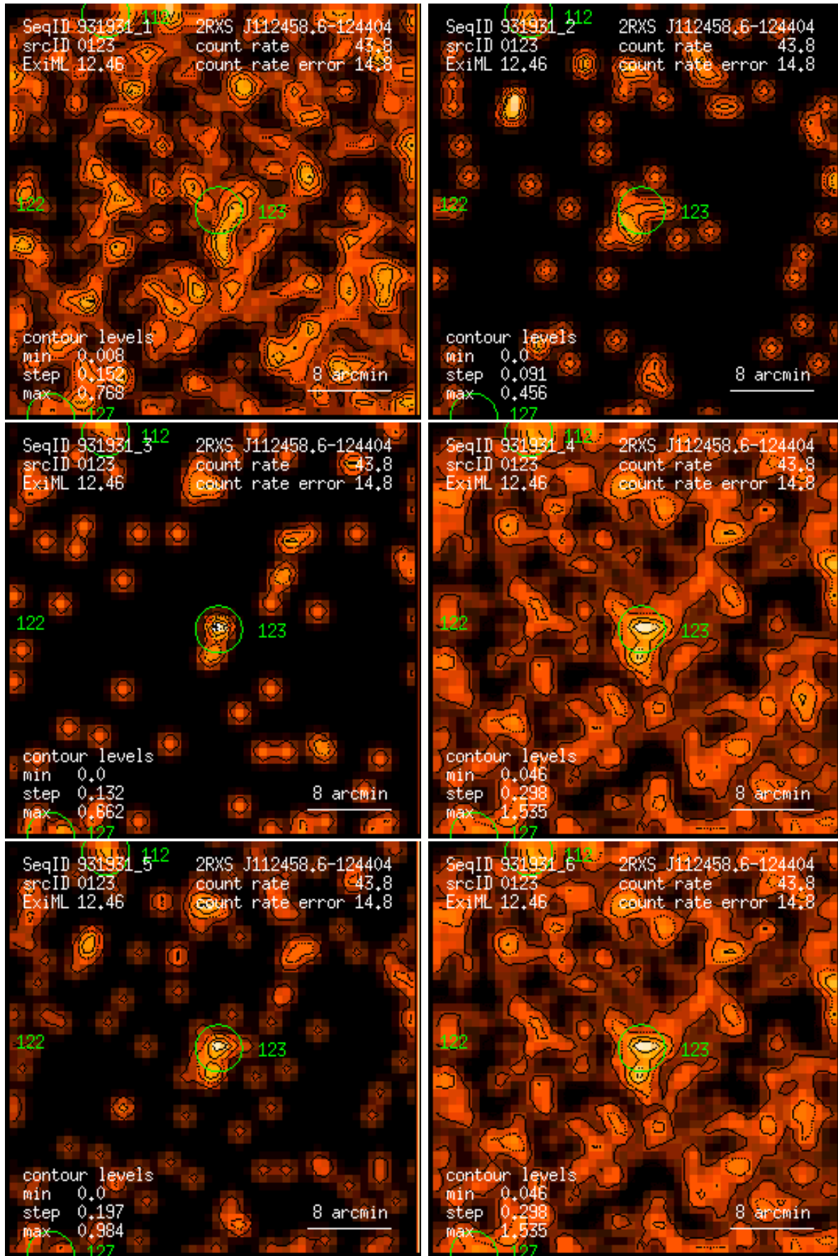
Figure 123: RASS 931931: detection 0123: band rate images, Gaussian filter: (1) PSPC channels 11 – 41, (2) 52 – 90, (3) 91 – 201, (4) 11 – 235, (5) 52 – 201, (6) 11 – 201. Broad band rates in counts/ks. Band rate contour levels in counts/ks/arcmin 2 .
