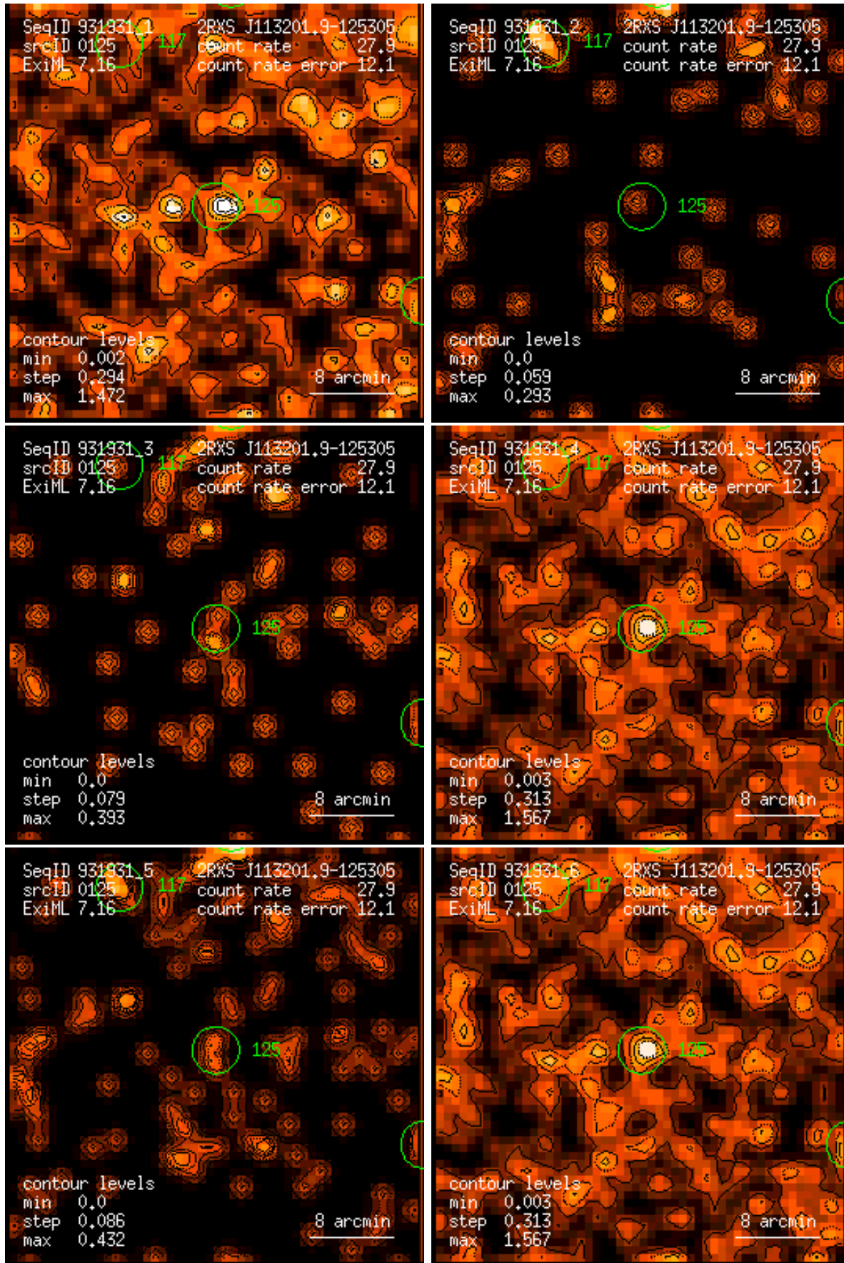
Figure 125: RASS 931931: detection 0125: band rate images, Gaussian filter: (1) PSPC channels 11 – 41, (2) 52 – 90, (3) 91 – 201, (4) 11 – 235, (5) 52 – 201, (6) 11 – 201. Broad band rates in counts/ks. Band rate contour levels in counts/ks/arcmin 2 .
