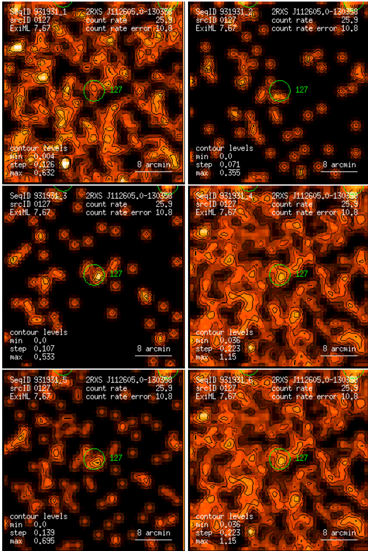
Figure 127: RASS 931931: detection 0127: band rate images, Gaussian filter: (1) PSPC channels 11 – 41, (2) 52 – 90, (3) 91 – 201, (4) 11 – 235, (5) 52 – 201, (6) 11 – 201. Broad band rates in counts/ks. Band rate contour levels in counts/ks/arcmin 2 .
