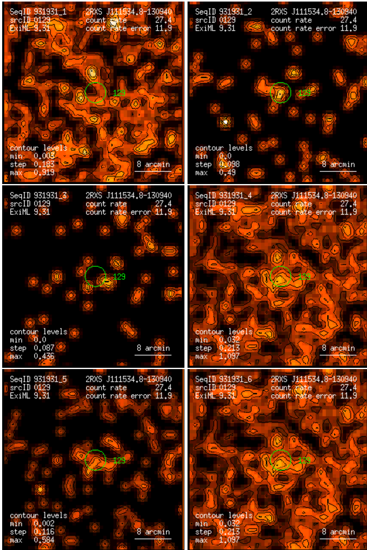
Figure 129: RASS 931931: detection 0129: band rate images, Gaussian filter: (1) PSPC channels 11 – 41, (2) 52 – 90, (3) 91 – 201, (4) 11 – 235, (5) 52 – 201, (6) 11 – 201. Broad band rates in counts/ks. Band rate contour levels in counts/ks/arcmin 2 .
