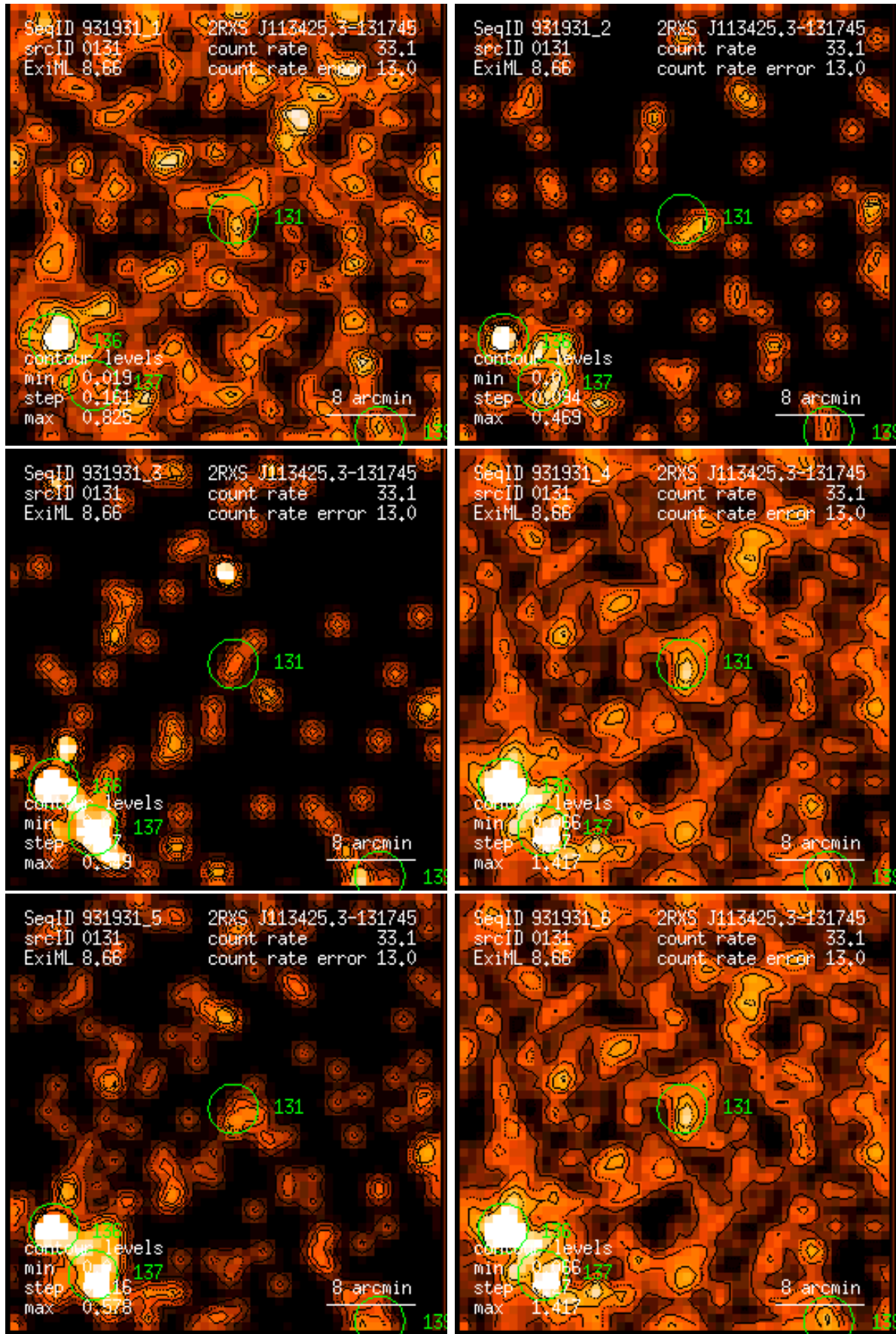
Figure 131: RASS 931931: detection 0131: band rate images, Gaussian filter: (1) PSPC channels 11 – 41, (2) 52 – 90, (3) 91 – 201, (4) 11 – 235, (5) 52 – 201, (6) 11 – 201. Broad band rates in counts/ks. Band rate contour levels in counts/ks/arcmin 2 .
