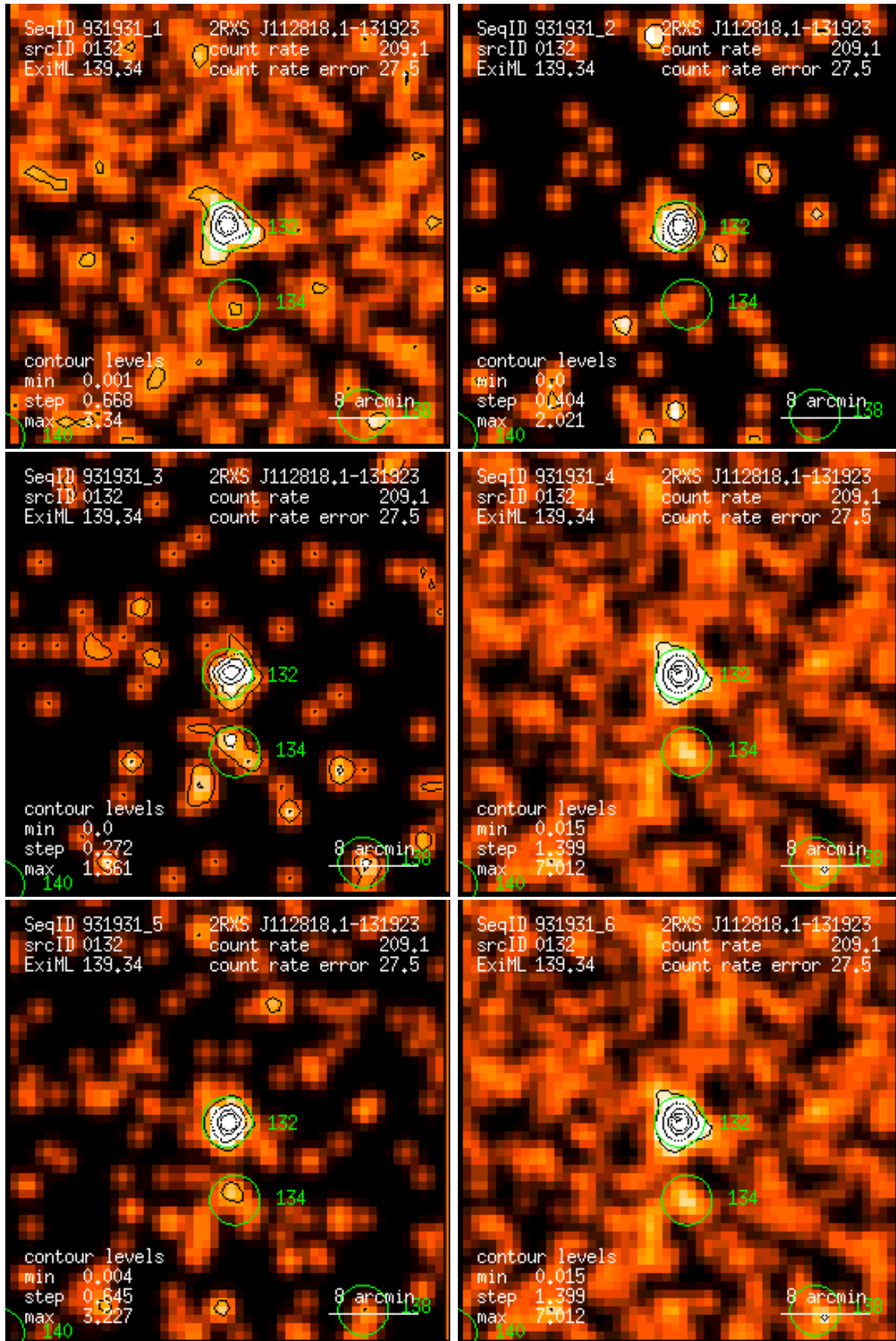
Figure 132: RASS 931931: detection 0132: band rate images, Gaussian filter: (1) PSPC channels 11 – 41, (2) 52 – 90, (3) 91 – 201, (4) 11 – 235, (5) 52 – 201, (6) 11 – 201. Broad band rates in counts/ks. Band rate contour levels in counts/ks/arcmin 2 .
