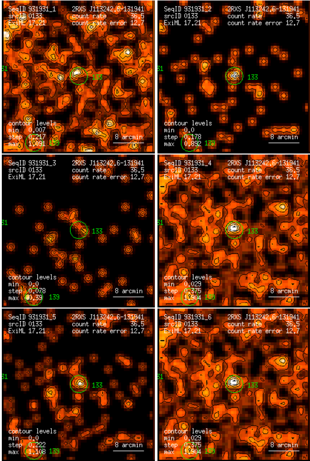
Figure 133: RASS 931931: detection 0133: band rate images, Gaussian filter: (1) PSPC channels 11 – 41, (2) 52 – 90, (3) 91 – 201, (4) 11 – 235, (5) 52 – 201, (6) 11 – 201. Broad band rates in counts/ks. Band rate contour levels in counts/ks/arcmin 2 .
