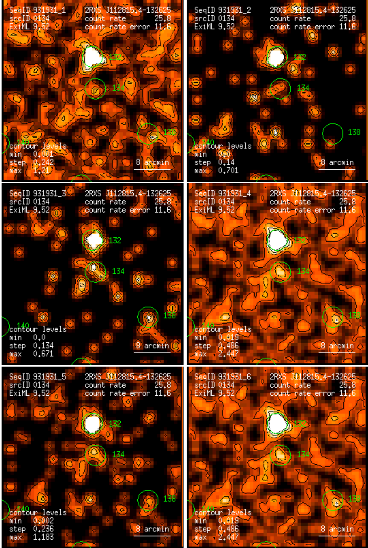
Figure 134: RASS 931931: detection 0134: band rate images, Gaussian filter: (1) PSPC channels 11 – 41, (2) 52 – 90, (3) 91 – 201, (4) 11 – 235, (5) 52 – 201, (6) 11 – 201. Broad band rates in counts/ks. Band rate contour levels in counts/ks/arcmin 2 .
