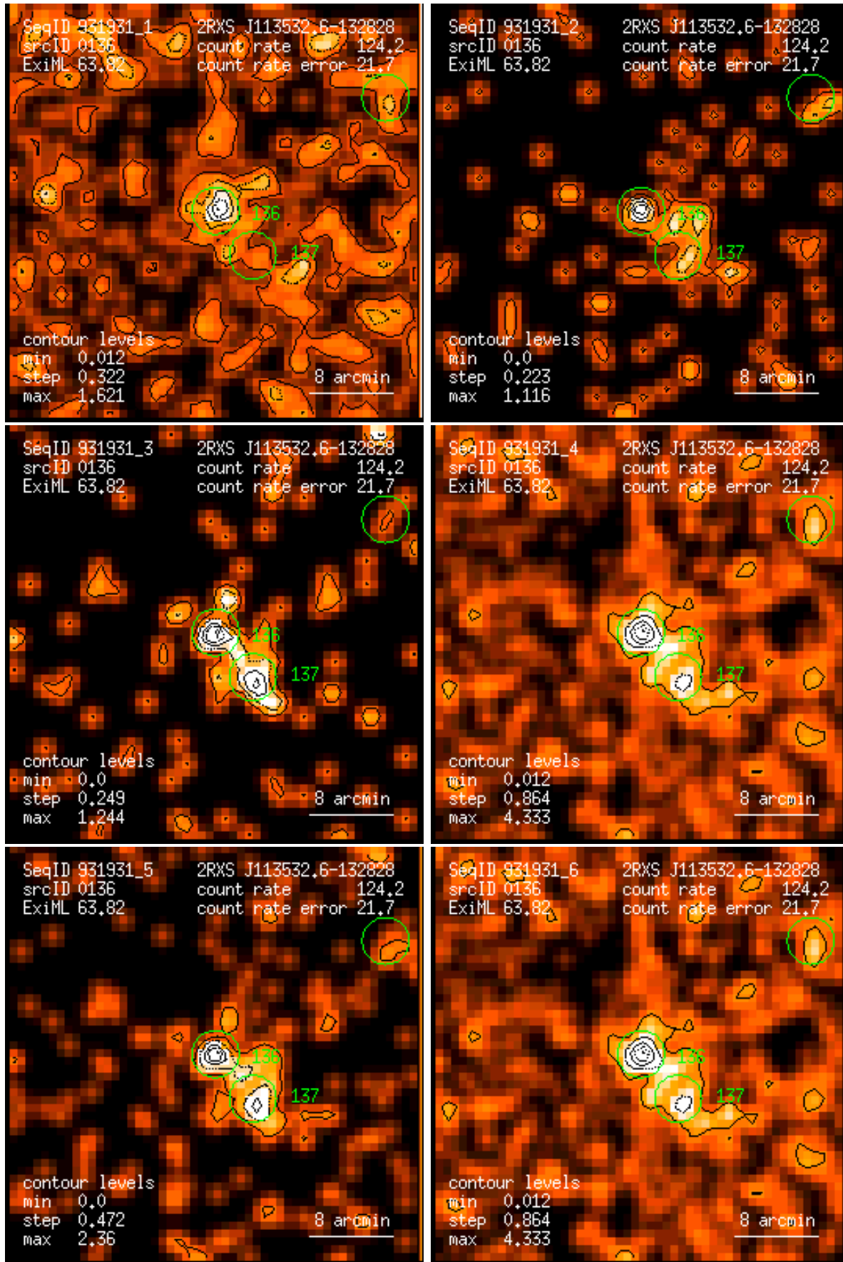
Figure 136: RASS 931931: detection 0136: band rate images, Gaussian filter: (1) PSPC channels 11 – 41, (2) 52 – 90, (3) 91 – 201, (4) 11 – 235, (5) 52 – 201, (6) 11 – 201. Broad band rates in counts/ks. Band rate contour levels in counts/ks/arcmin 2 .
