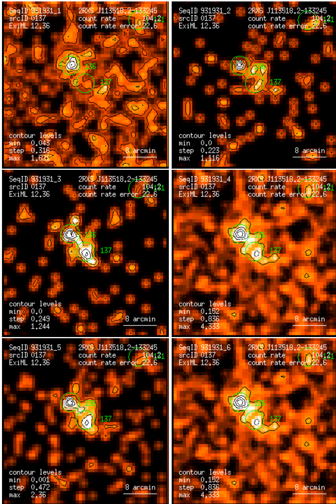
Figure 137: RASS 931931: detection 0137: band rate images, Gaussian filter: (1) PSPC channels 11 – 41, (2) 52 – 90, (3) 91 – 201, (4) 11 – 235, (5) 52 – 201, (6) 11 – 201. Broad band rates in counts/ks. Band rate contour levels in counts/ks/arcmin 2 .
