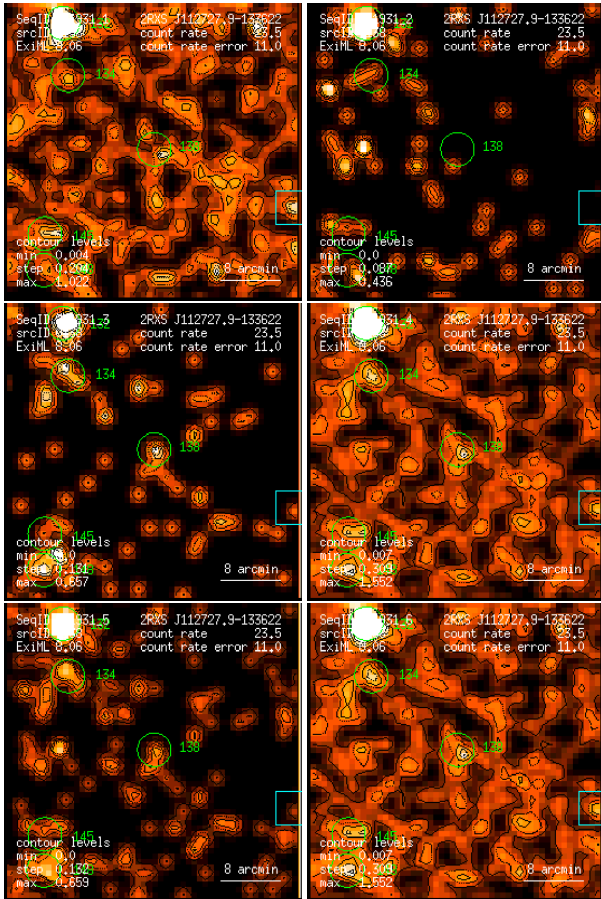
Figure 138: RASS 931931: detection 0138: band rate images, Gaussian filter: (1) PSPC channels 11 – 41, (2) 52 – 90, (3) 91 – 201, (4) 11 – 235, (5) 52 – 201, (6) 11 – 201. Broad band rates in counts/ks. Band rate contour levels in counts/ks/arcmin 2 .
