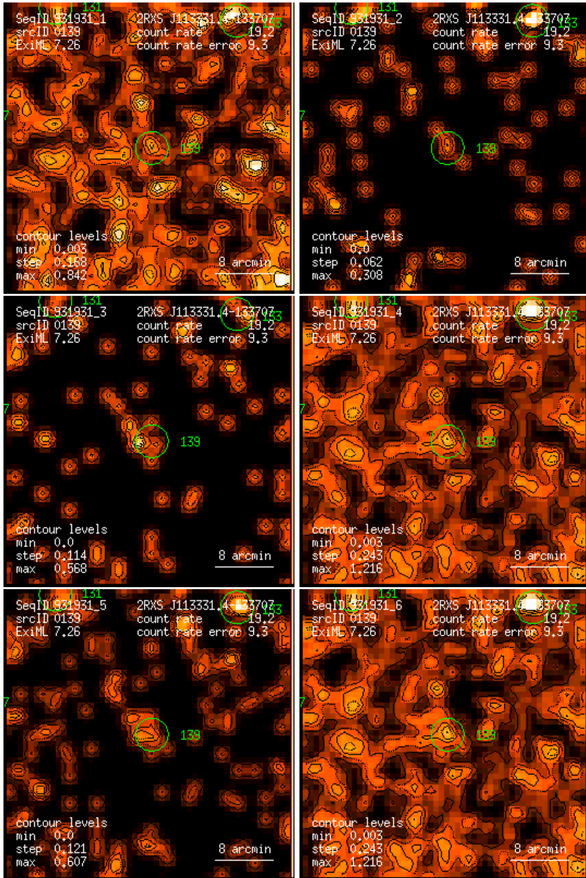
Figure 139: RASS 931931: detection 0139: band rate images, Gaussian filter: (1) PSPC channels 11 – 41, (2) 52 – 90, (3) 91 – 201, (4) 11 – 235, (5) 52 – 201, (6) 11 – 201. Broad band rates in counts/ks. Band rate contour levels in counts/ks/arcmin 2 .
