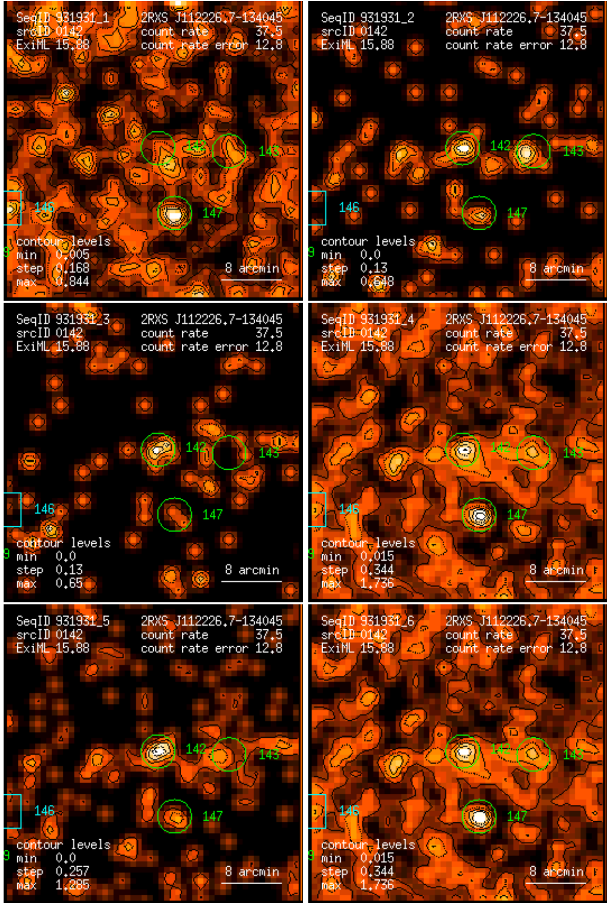
Figure 142: RASS 931931: detection 0142: band rate images, Gaussian filter: (1) PSPC channels 11 – 41, (2) 52 – 90, (3) 91 – 201, (4) 11 – 235, (5) 52 – 201, (6) 11 – 201. Broad band rates in counts/ks. Band rate contour levels in counts/ks/arcmin 2 .
