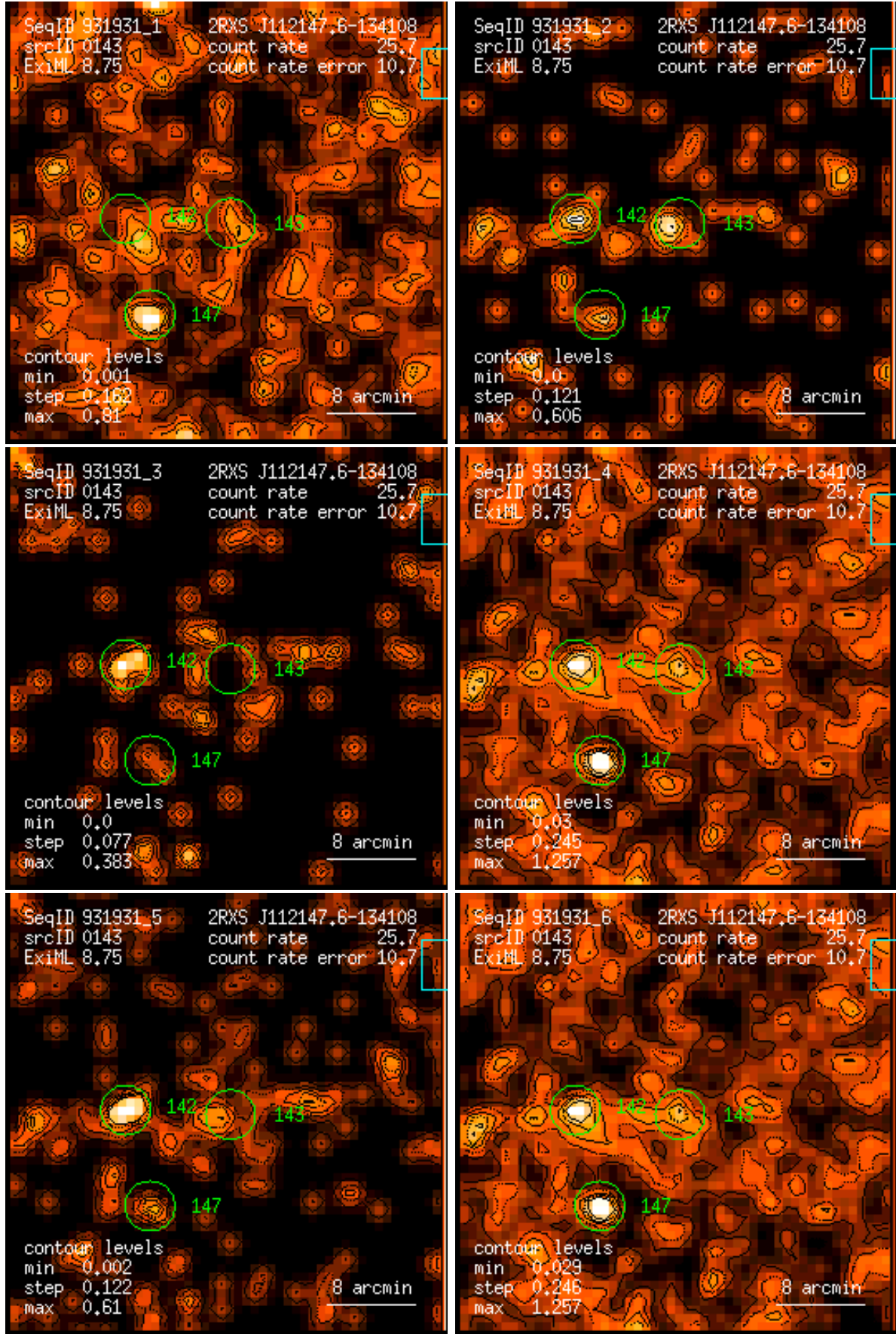
Figure 143: RASS 931931: detection 0143: band rate images, Gaussian filter: (1) PSPC channels 11 – 41, (2) 52 – 90, (3) 91 – 201, (4) 11 – 235, (5) 52 – 201, (6) 11 – 201. Broad band rates in counts/ks. Band rate contour levels in counts/ks/arcmin 2 .
