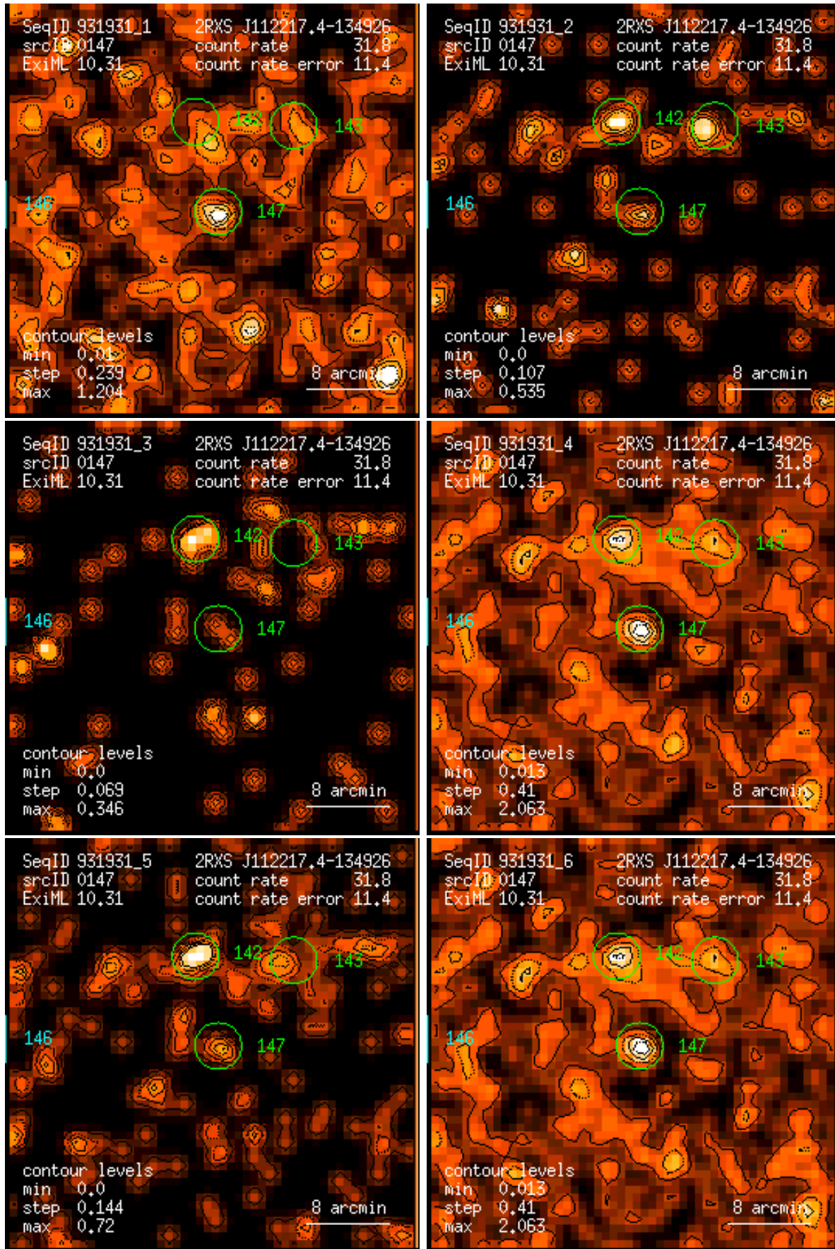
Figure 147: RASS 931931: detection 0147: band rate images, Gaussian filter: (1) PSPC channels 11 – 41, (2) 52 – 90, (3) 91 – 201, (4) 11 – 235, (5) 52 – 201, (6) 11 – 201. Broad band rates in counts/ks. Band rate contour levels in counts/ks/arcmin 2 .
