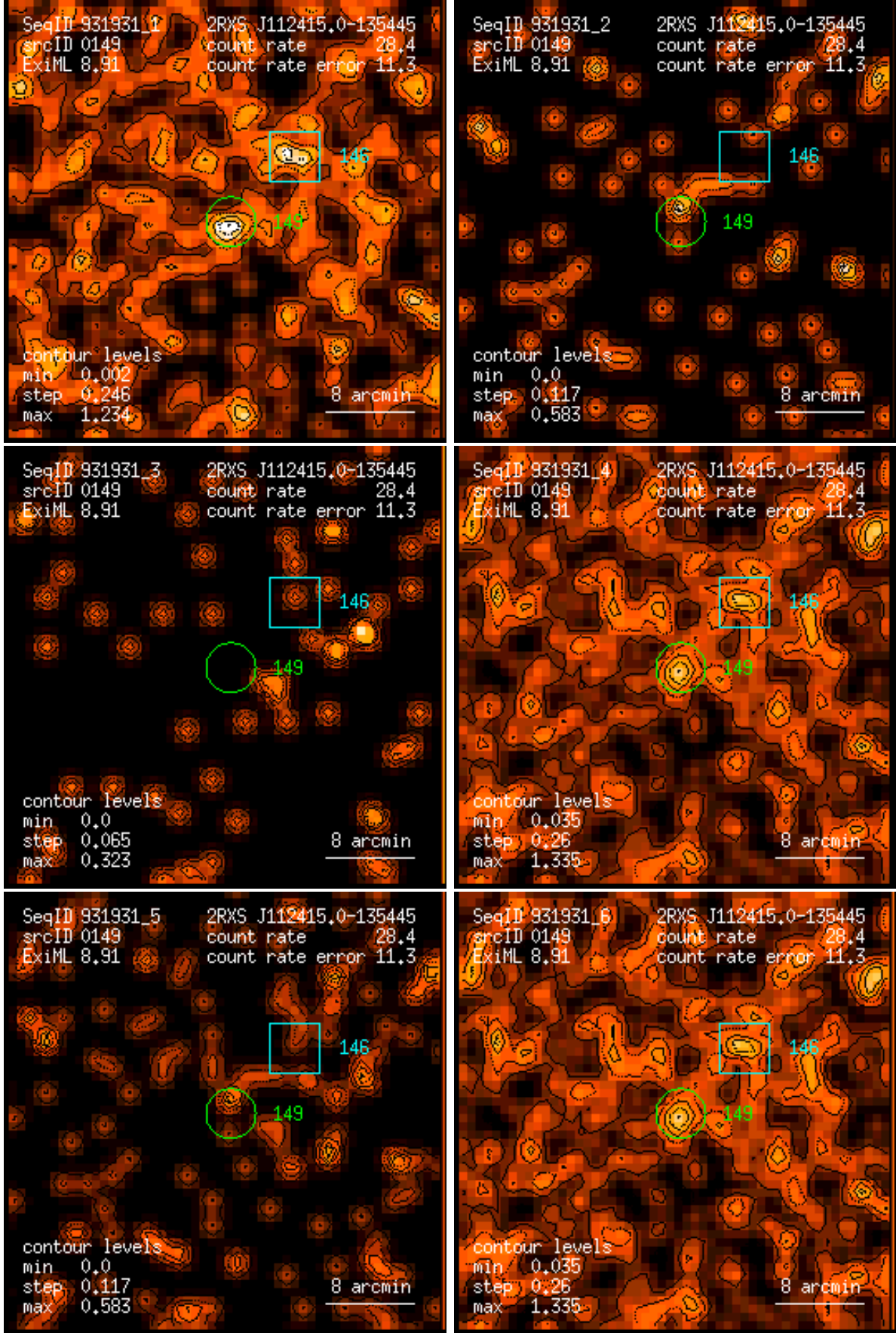
Figure 149: RASS 931931: detection 0149: band rate images, Gaussian filter: (1) PSPC channels 11 – 41, (2) 52 – 90, (3) 91 – 201, (4) 11 – 235, (5) 52 – 201, (6) 11 – 201. Broad band rates in counts/ks. Band rate contour levels in counts/ks/arcmin 2 .
